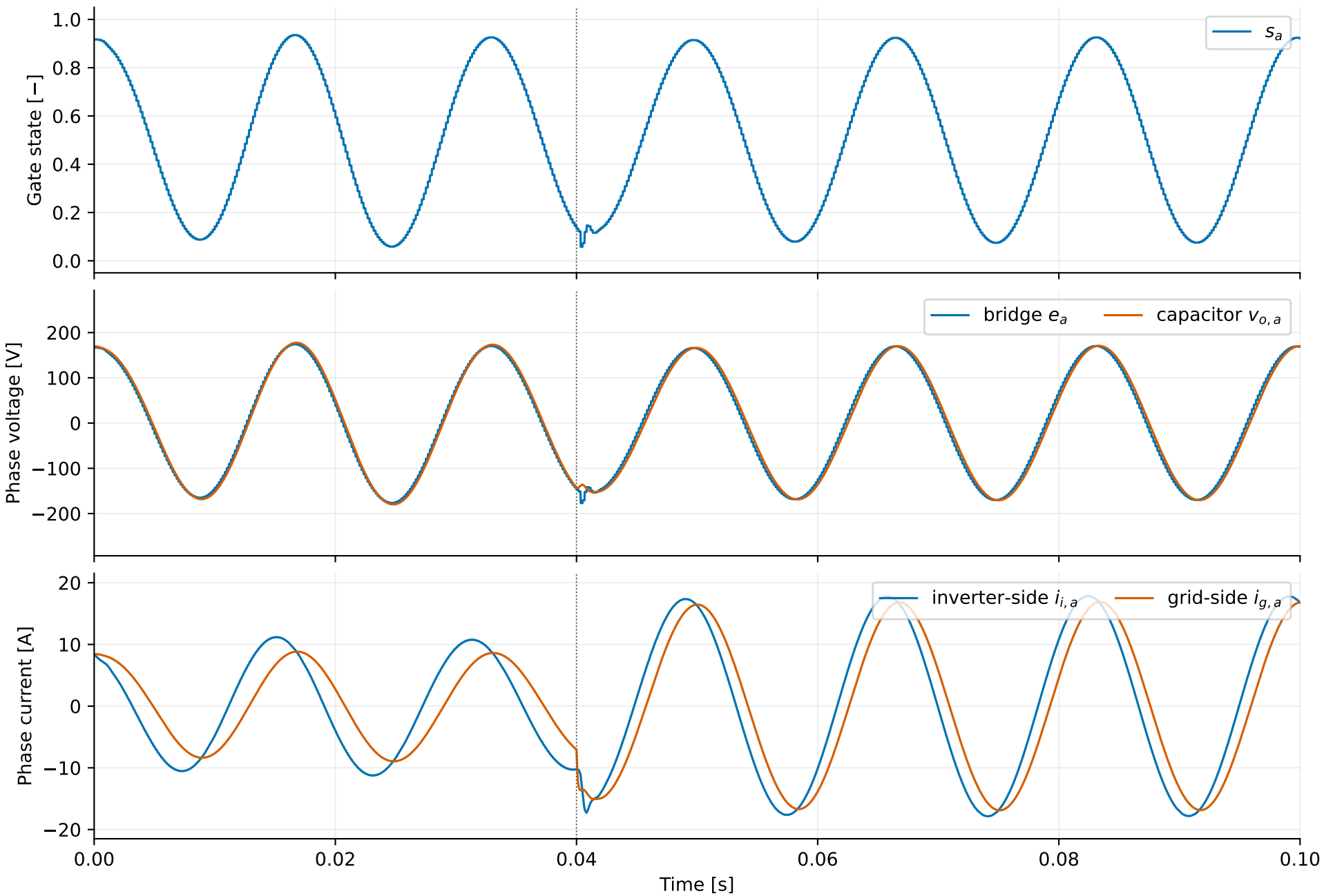
6 kHz PWM, islanded voltage control, \mu = 240
