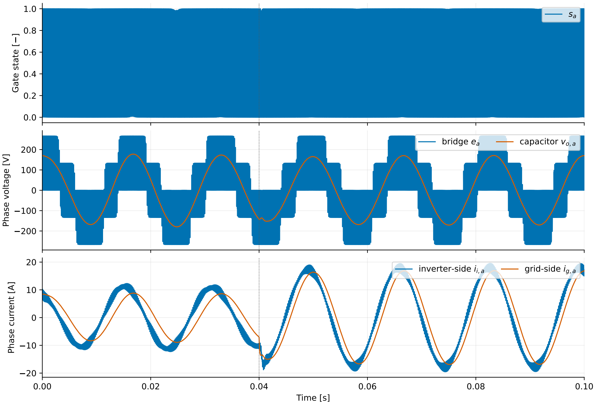
6 kHz PWM, islanded voltage control, \mu = 1e + 06
