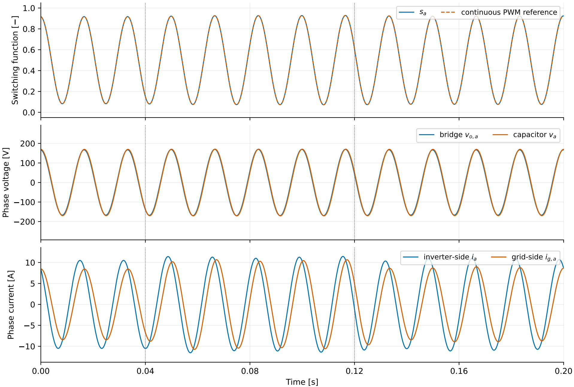
6000 Hz PWM, PLL-synchronized voltage control, \mu = 240 \text{ s}^{-1}
