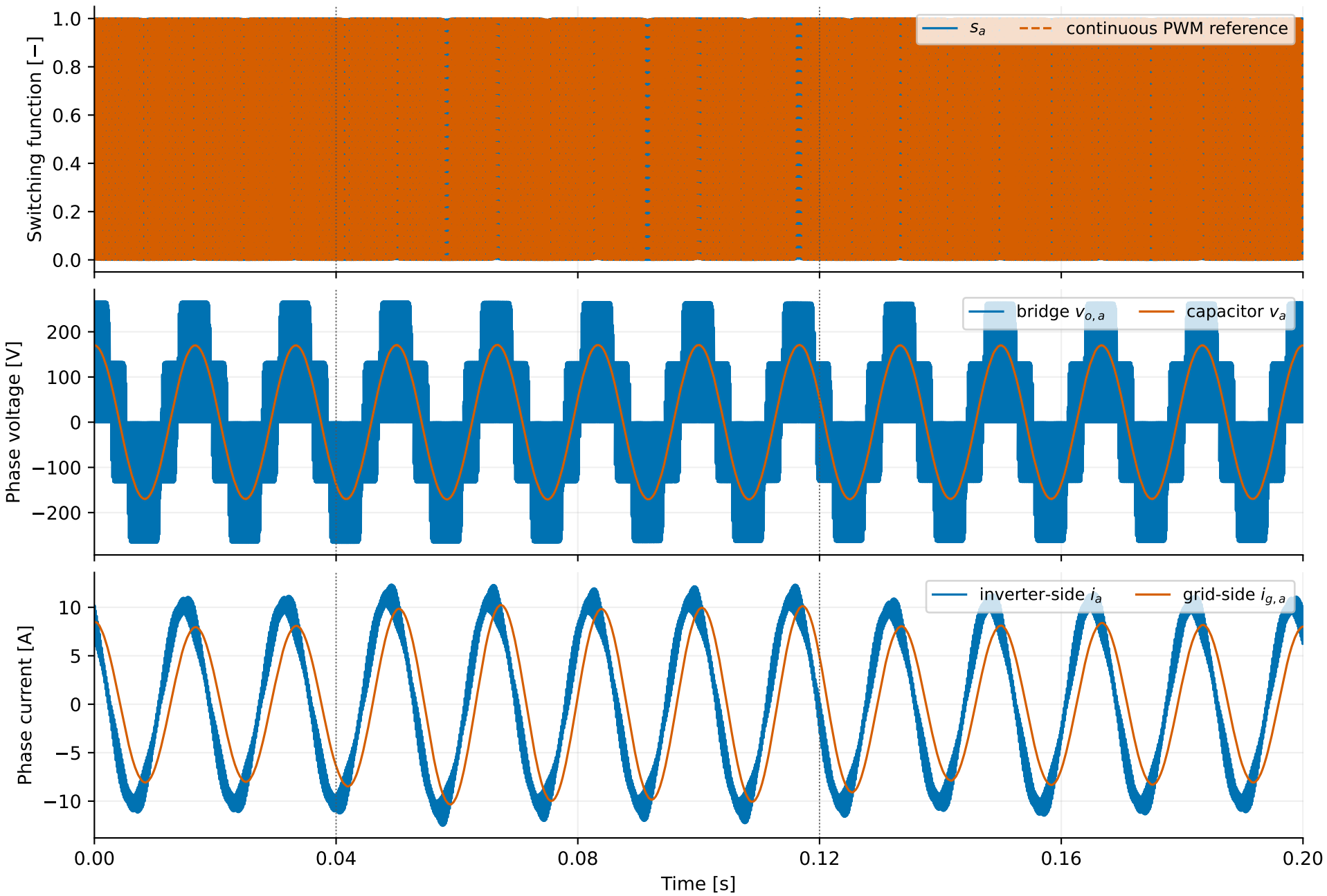
6000 Hz PWM, PLL-synchronized voltage control, \mu = 10^6 \text{ s}^{-1}
