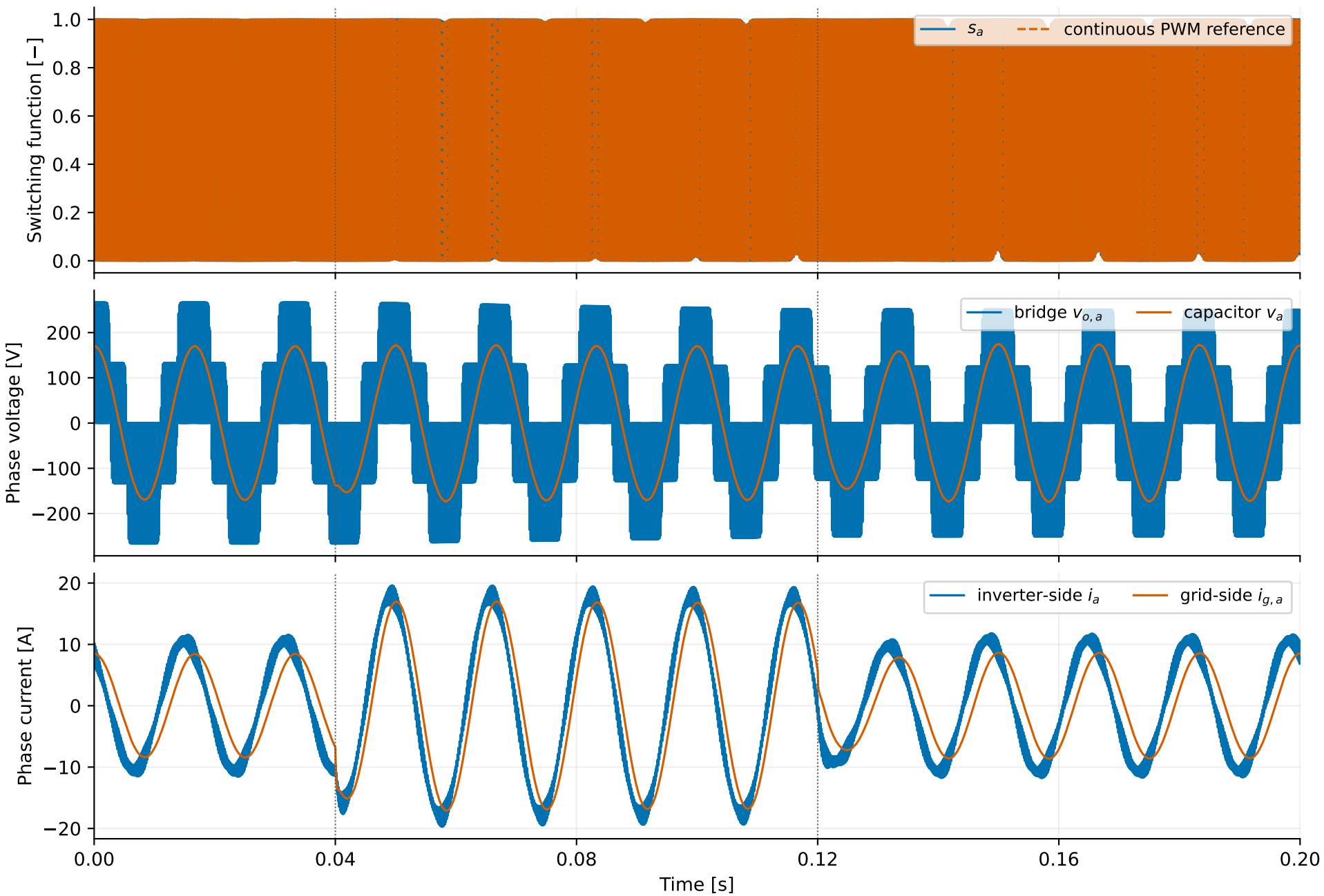
6000 Hz PWM, islanded voltage control, \mu = 1e + 06
