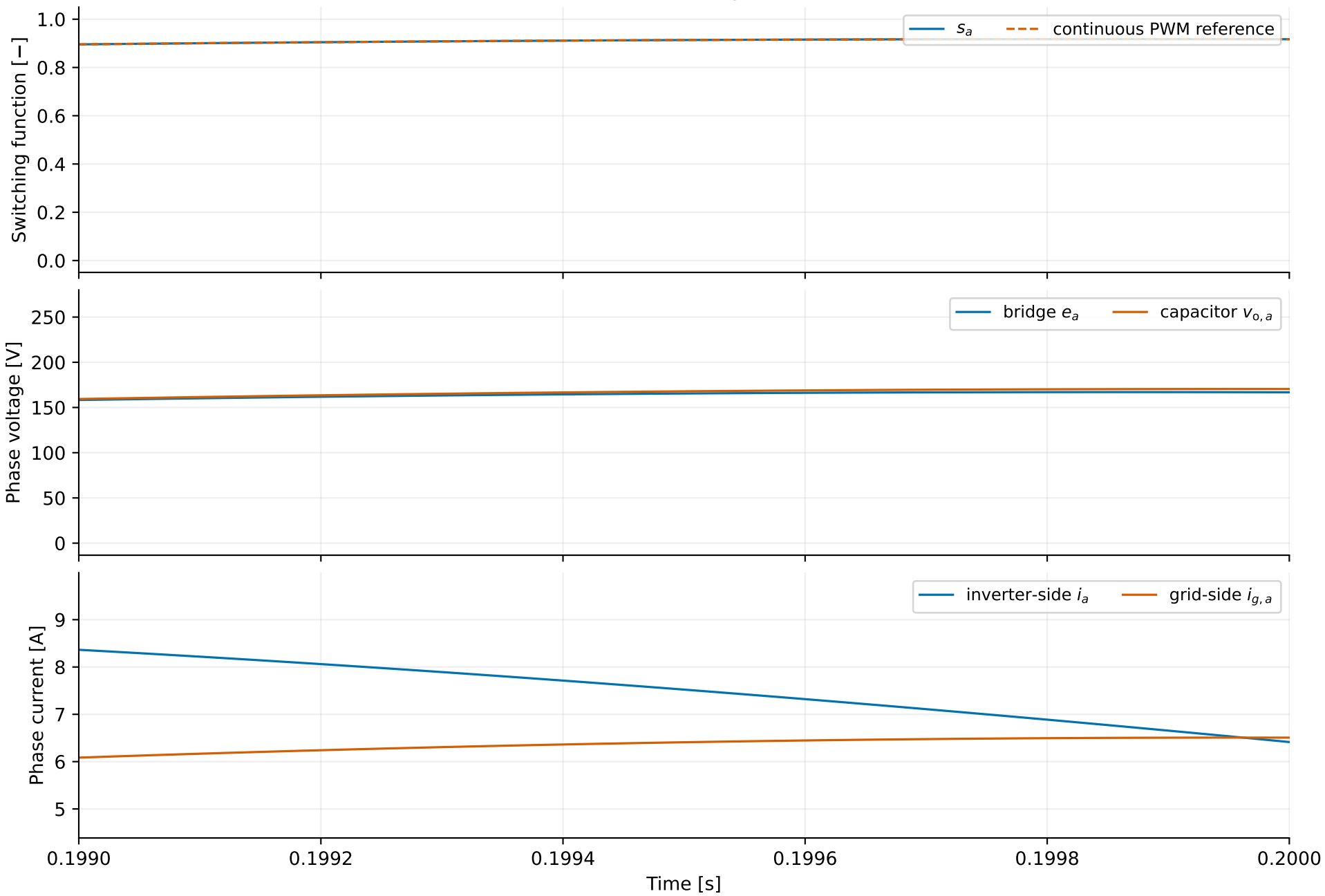
6000 Hz PWM, GFL, \mu = 240 \text{ s}^{-1}
