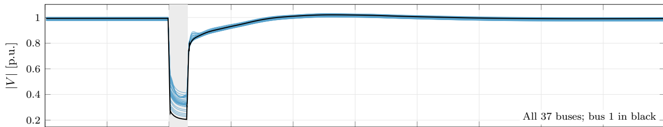
(b) GridKit PhasorDynamics; fault cleared at 1.15 s
