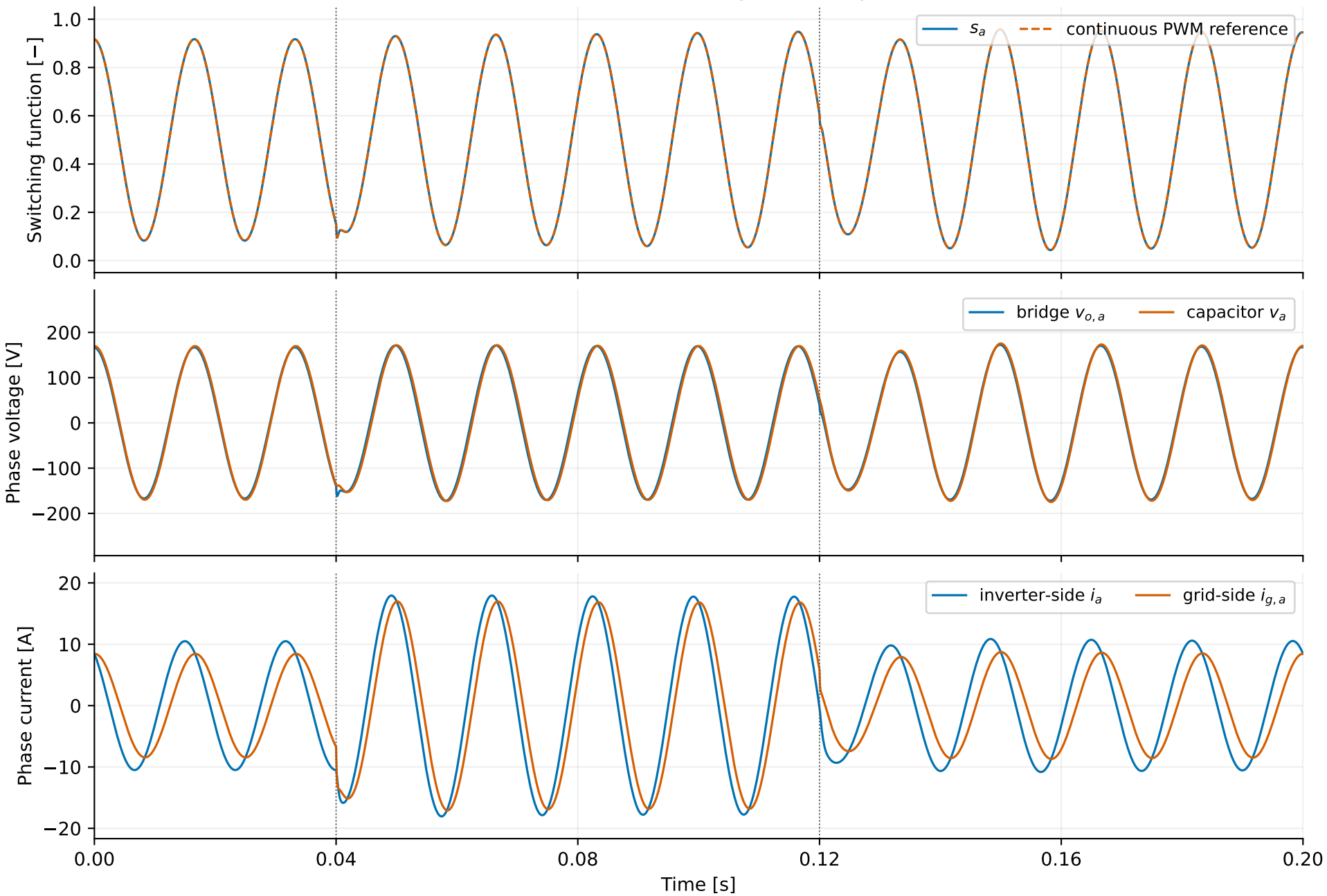
6000 Hz PWM, islanded voltage control, \mu = 240 \text{ s}^{-1}
