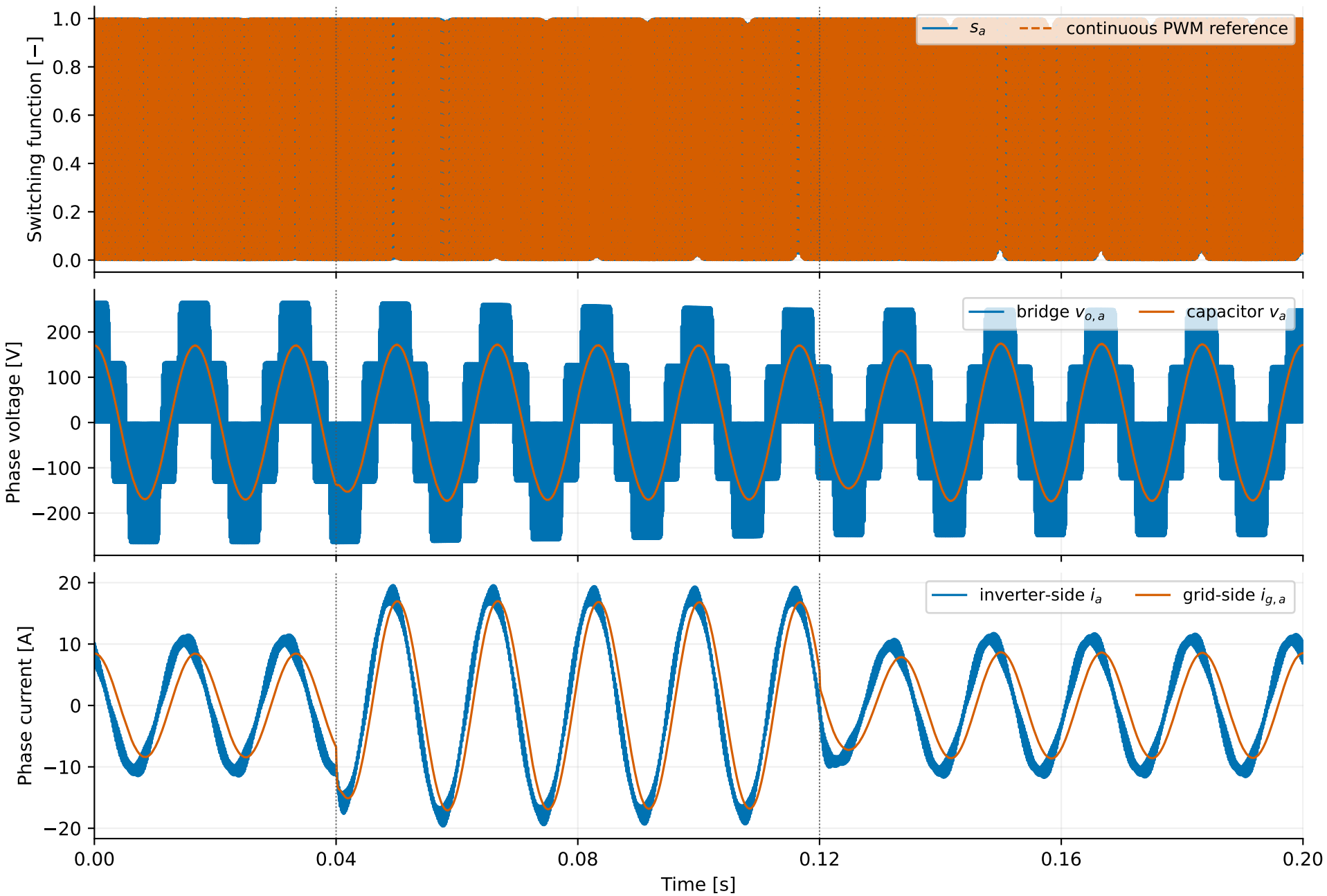
6000 Hz PWM, islanded voltage control, \mu = 10^6 \text{ s}^{-1}
