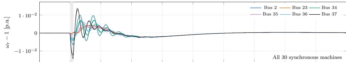
(b) PowerWorld reference; fault cleared at 1.15 s
