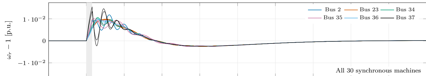
(c) EMT minus PowerWorld: range across channels
