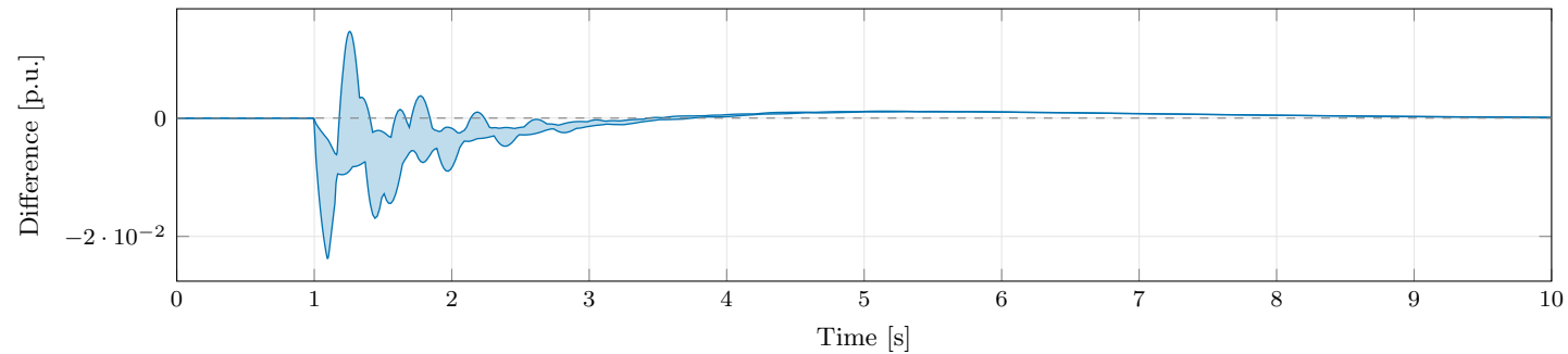
(c) EMT minus PowerWorld: range across channels
