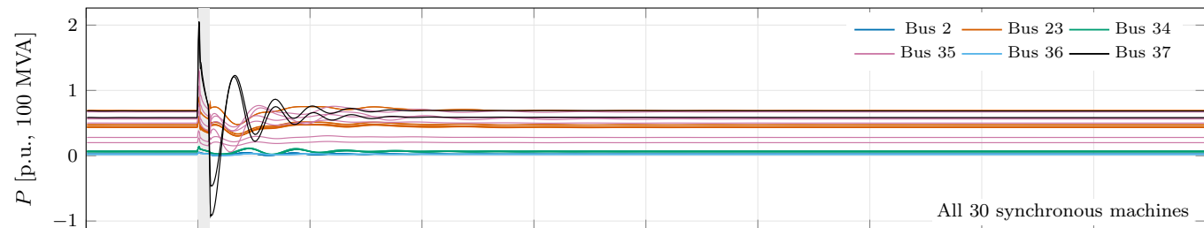
(b) PowerWorld reference; fault cleared at 1.15 s
