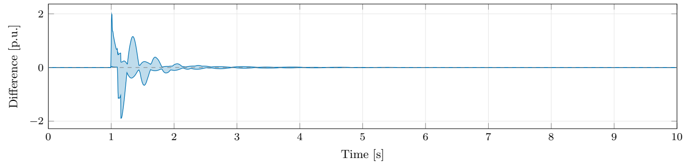
(c) EMT minus PowerWorld: range across channels
