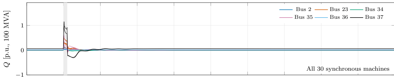
(b) PowerWorld reference; fault cleared at 1.15 s
