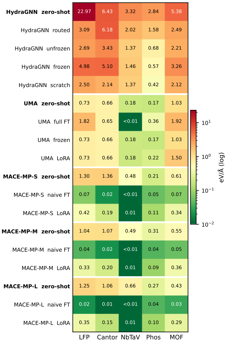
(a) Force MAE (eV/Å)
