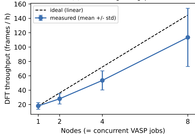
(a) DFT-labelling throughput
