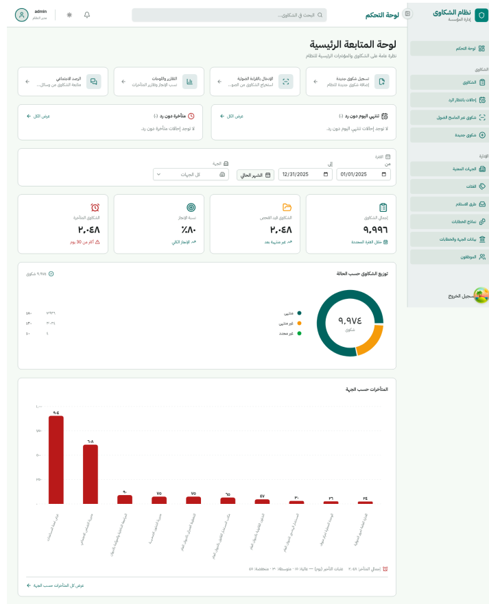
Screenshot: Dashboard
