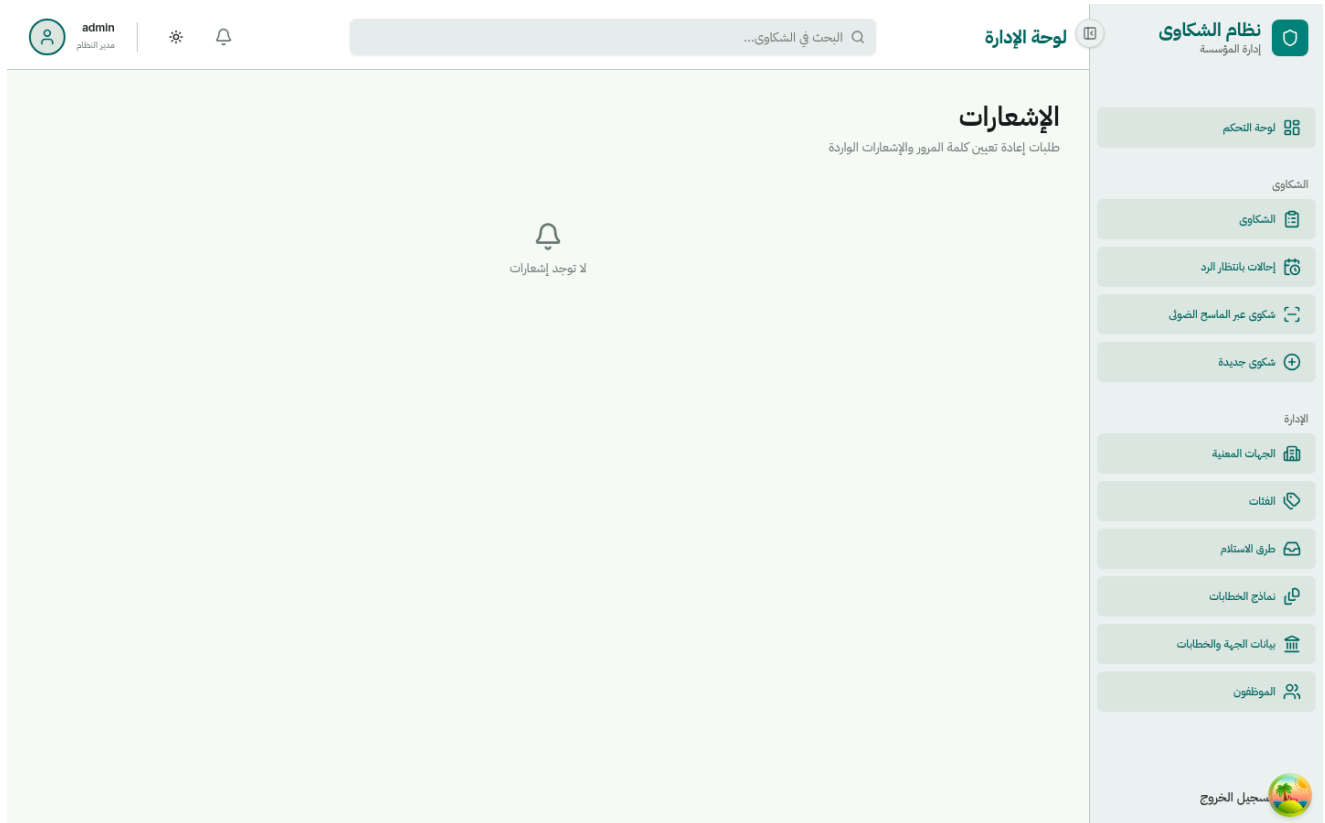
Screenshot: Notifications
