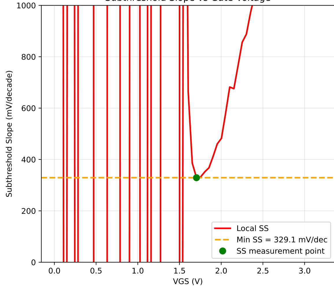
Subthreshold Slope vs Gate Voltage
