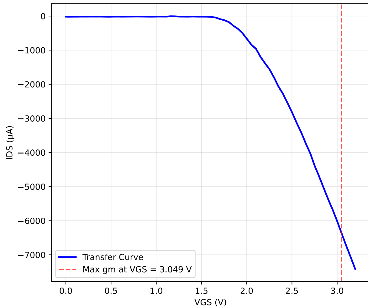
Transfer Characteristics (Drain = 1.0V)
