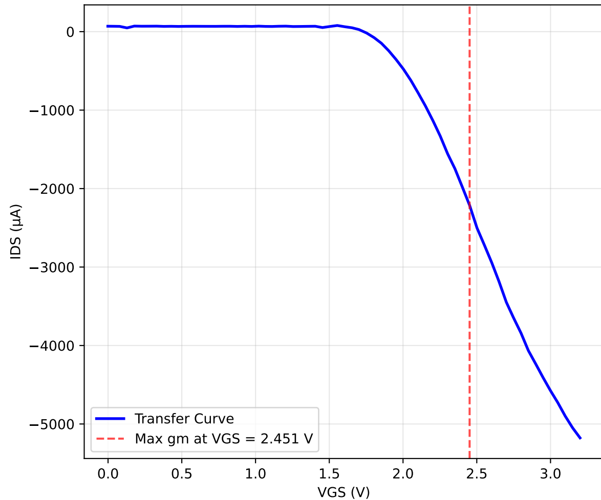
Transfer Characteristics (Drain = 2.0V)
