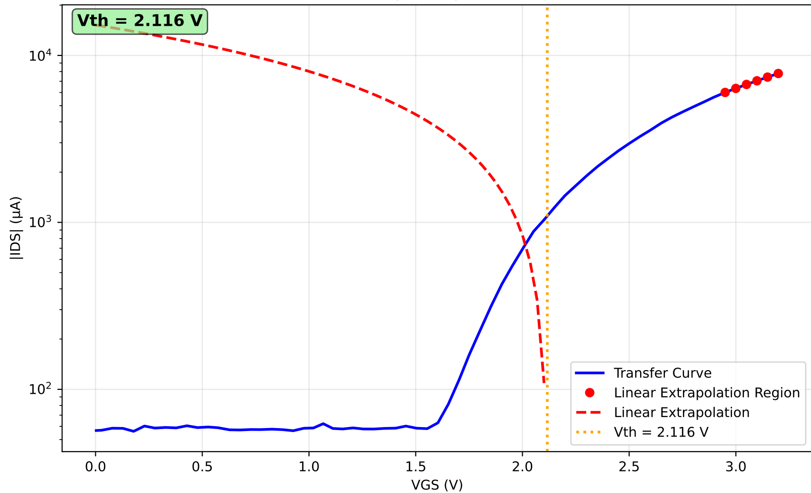
Threshold Voltage Analysis (Drain = 0.5V)
