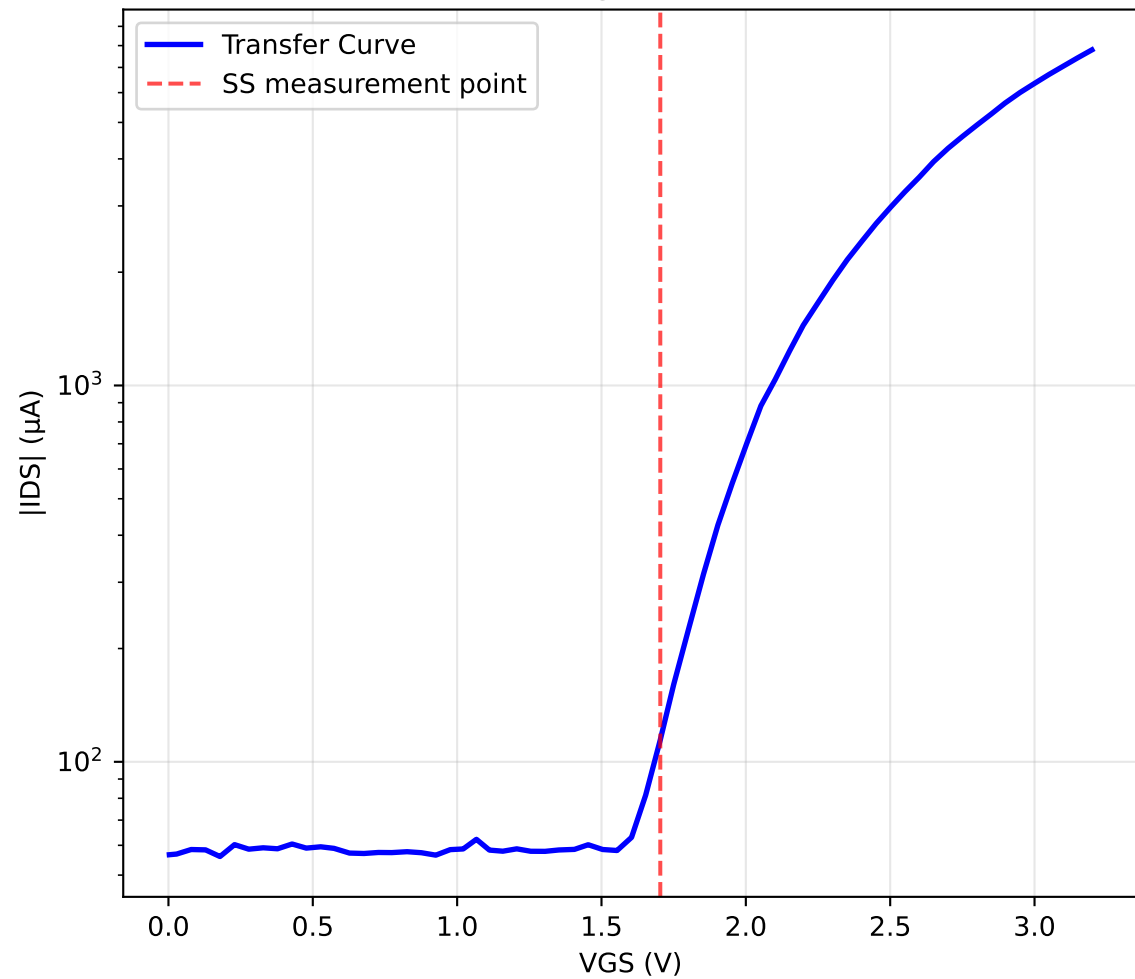
Transfer Curve (Log Scale) - Drain = 0.5V
