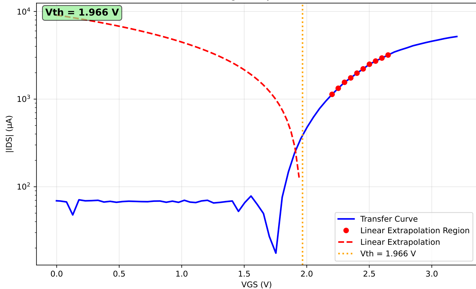
Threshold Voltage Analysis (Drain = 2.0V)
