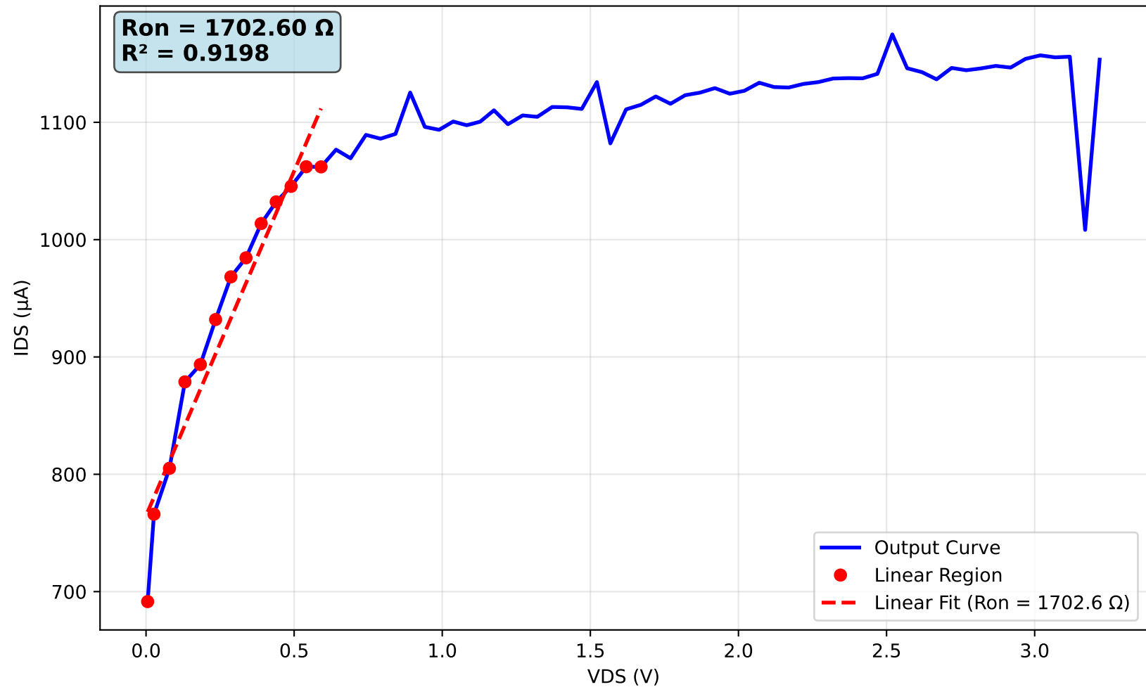
Channel Resistance Analysis (Gate = 1.0V)
