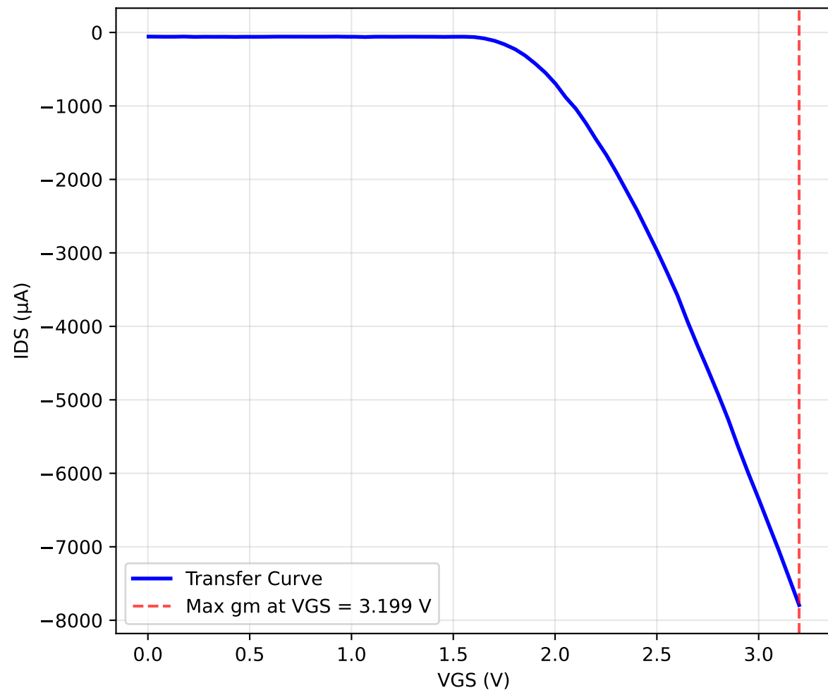
Transfer Characteristics (Drain = 0.5V)
