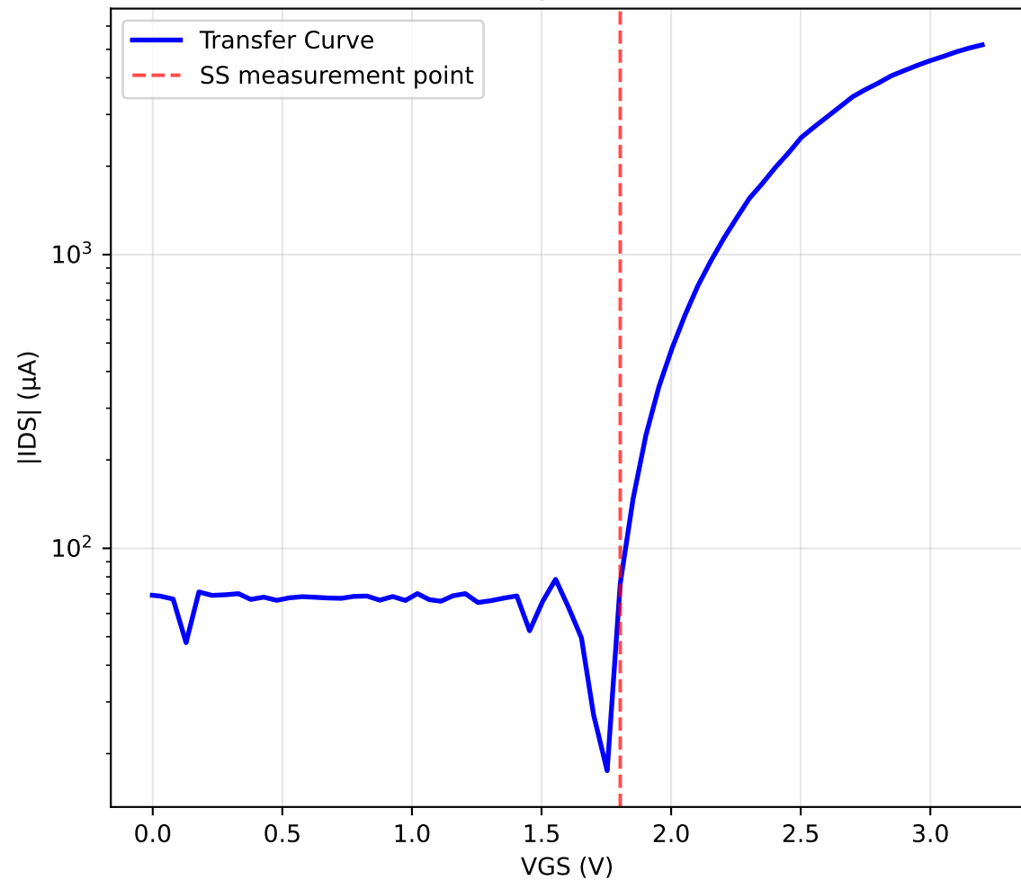
Transfer Curve (Log Scale) - Drain = 2.0V
