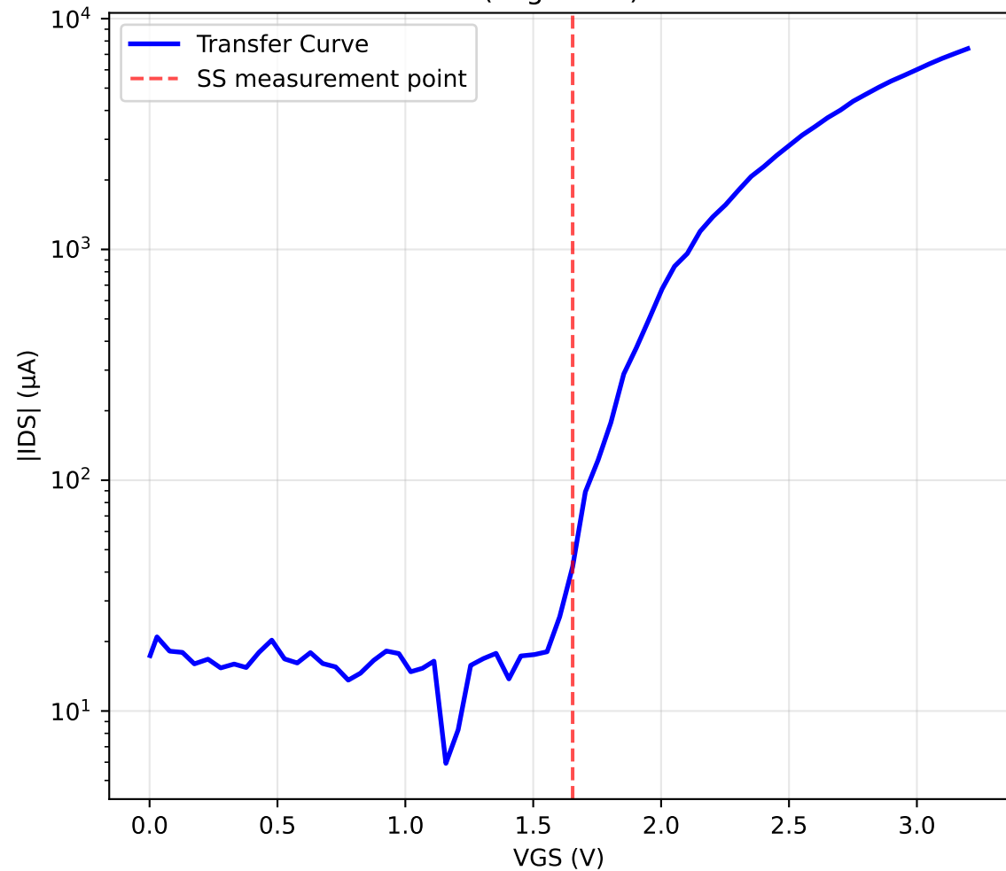
Transfer Curve (Log Scale) - Drain = 1.0V
