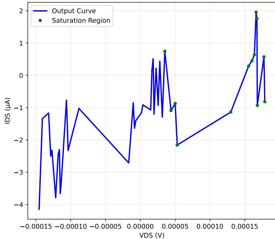
Output Conductance Analysis (Gate = 0.0V)
