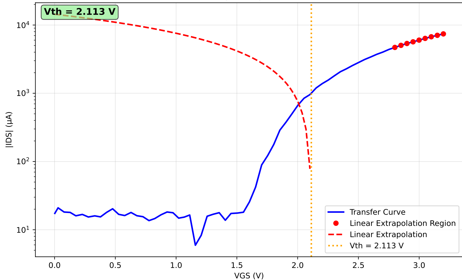
Threshold Voltage Analysis (Drain = 1.0V)
