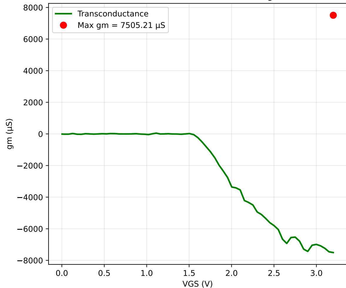
Transconductance vs Gate Voltage
