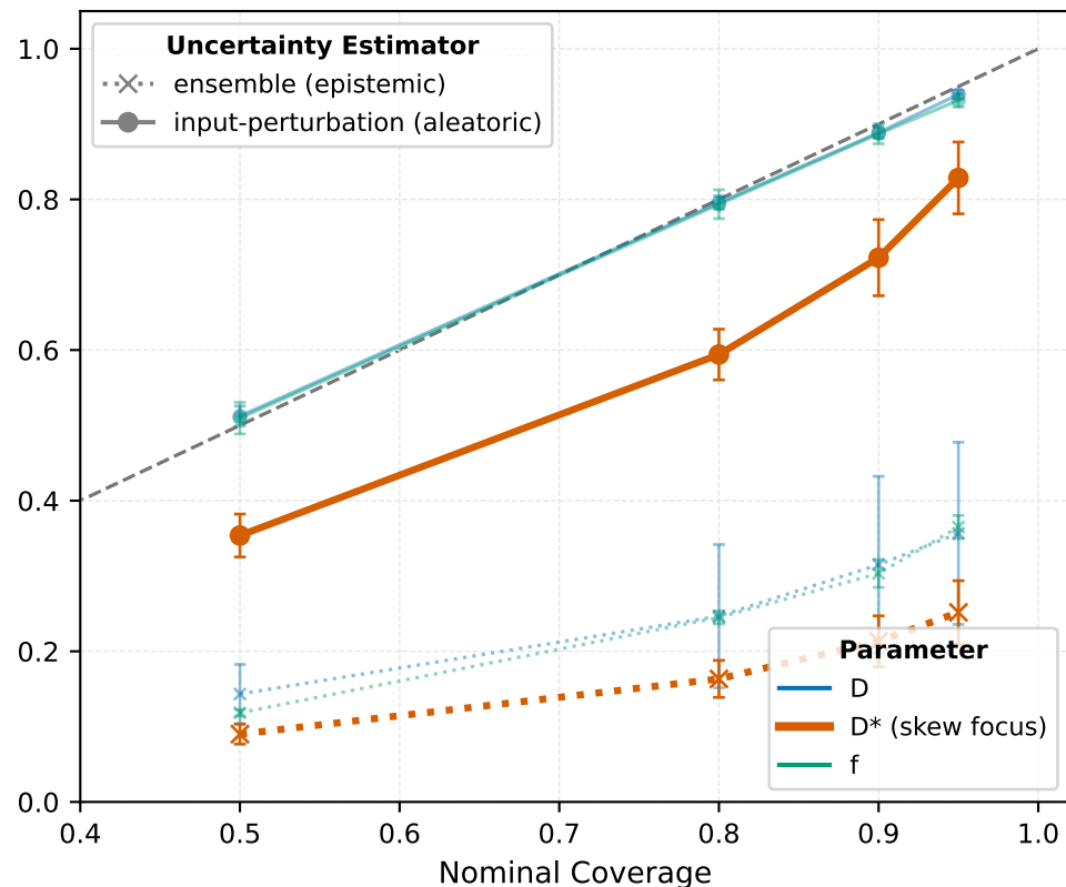
Deep-Learning Paradigm (Super_IVIM_DC)
