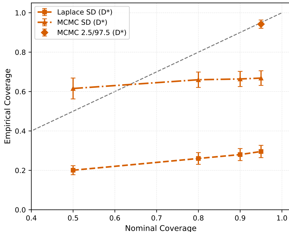
Bayesian Paradigm (D* Calibration)
