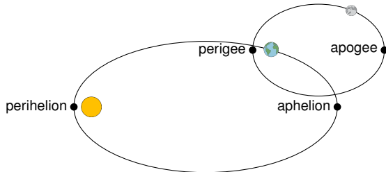
Elliptical orbits and their parameters.
