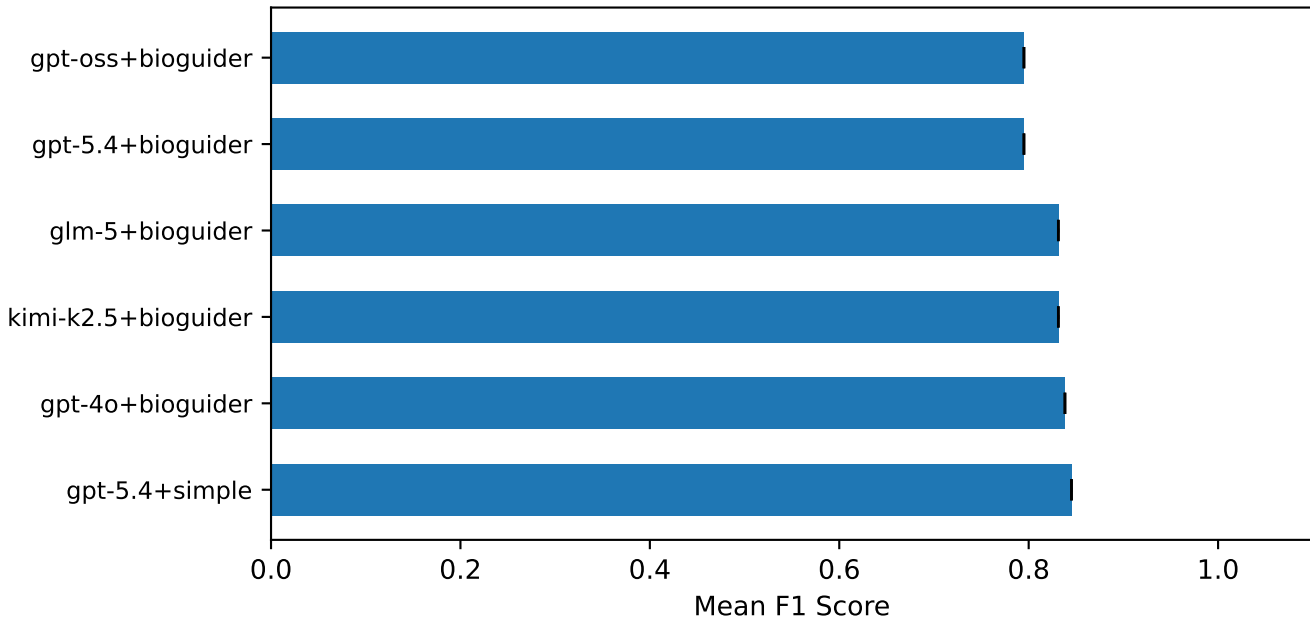
Average F1 Score by Model ( \pm 95\% CI)
