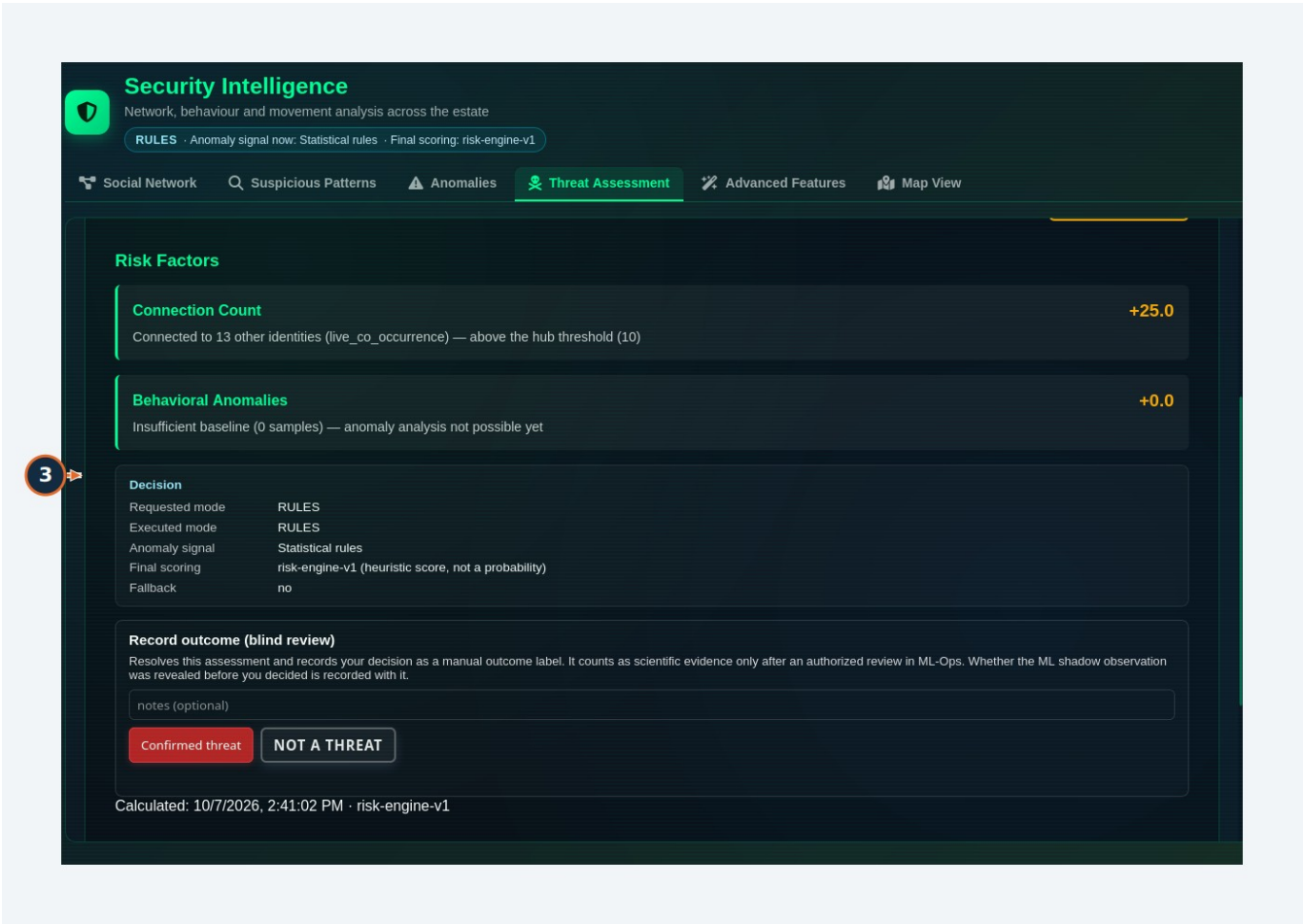
Figure 62. Steps 3. Read a persisted rules-based assessment with its limitations.
