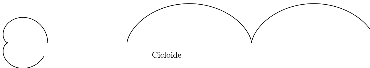
Cardioide r = 1 + \cos \theta
