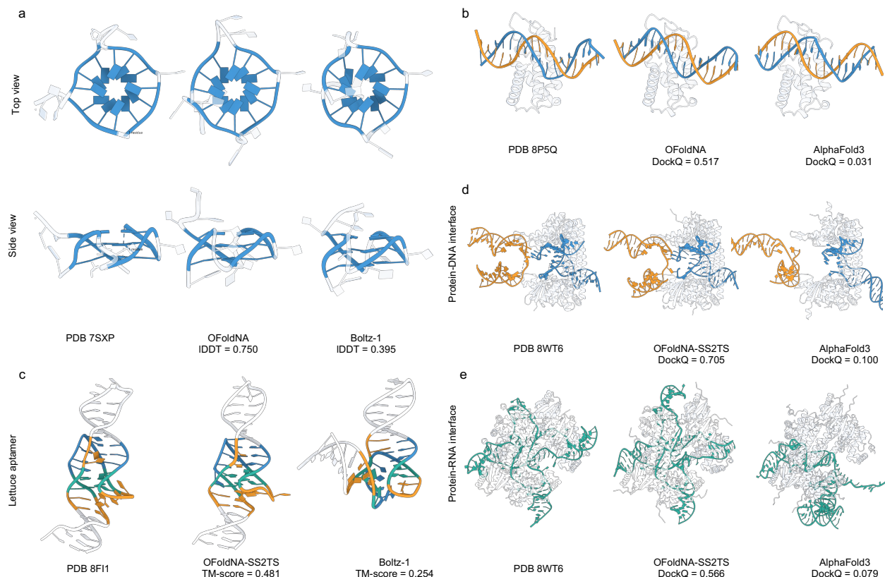
Figure 3 Representative structure predictions from OFoldNA and OFoldNA-SS2TS. a , Experimental structure of the 22-nucleotide G8U variant of the NRAS 5'-UTR RNA G-quadruplex (PDB ID: 7SXP), shown in top and side views, together with predictions from OFoldNA and Boltz-1. b , Experimental structure of the Arabidopsis thaliana ALOG domain-DNA complex (PDB ID: 8P5Q) and predictions from OFoldNA and AlphaFold 3. c , Experimental structure of the 53-nucleotide Lettuce C20G DNA aptamer bound to DFHO (PDB ID: 8FI1) and predictions from OFoldNA-SS2TS and Boltz-1. d,e , Protein-DNA ( d ) and protein-RNA ( e ) interfaces in the pre-strand-exchange IS621 recombinase complex containing bridge RNA, target DNA and donor DNA (PDB ID: 8WT6), together with predictions from OFoldNA-SS2TS and AlphaFold 3. OFoldNA-SS2TS denotes predictions generated using externally supplied SS information.
