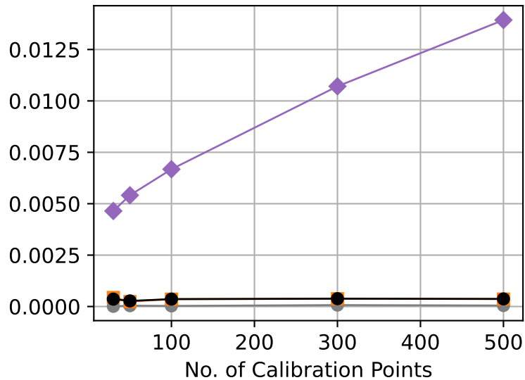
Dimension d = 10
