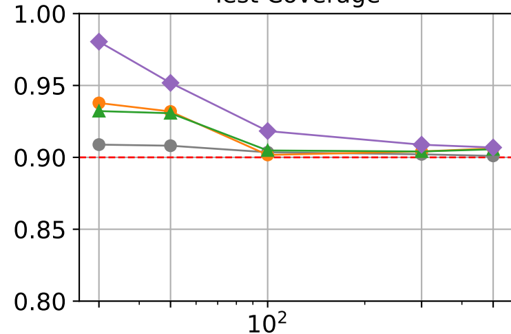
Test Coverage
