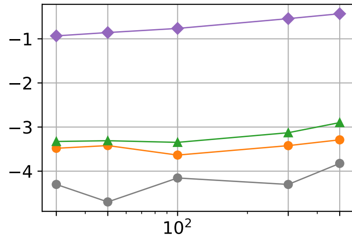
Runtime (Log10)
