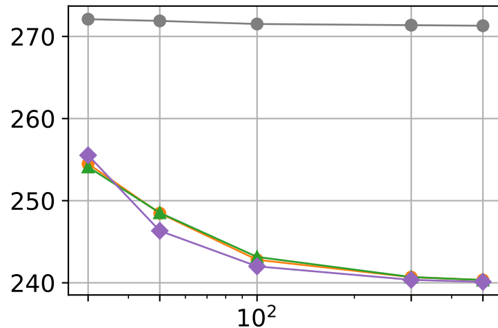
Volume (Log10)
