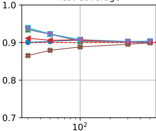
Test Coverage
