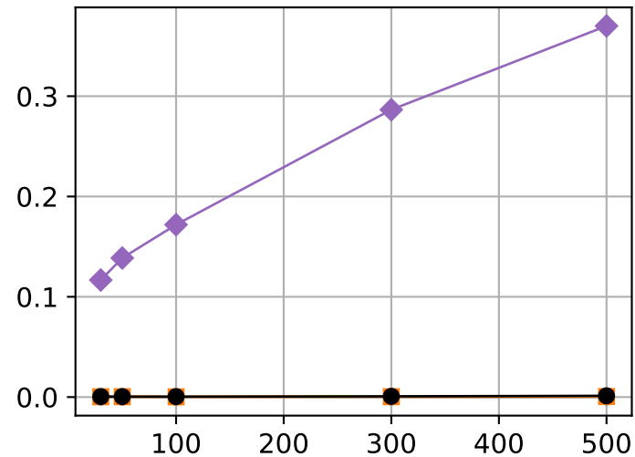
Dimension d = 100
