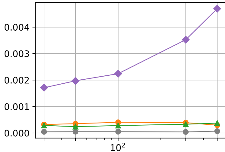
Runtime
