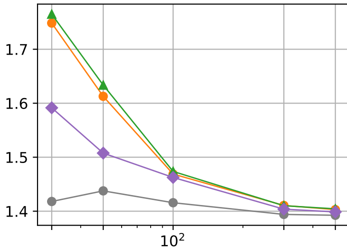
Volume (Log10)
