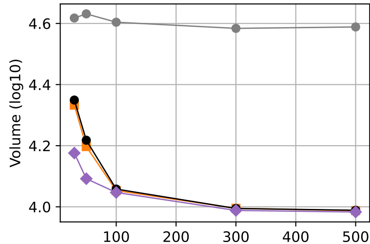
Dimension d = 4
