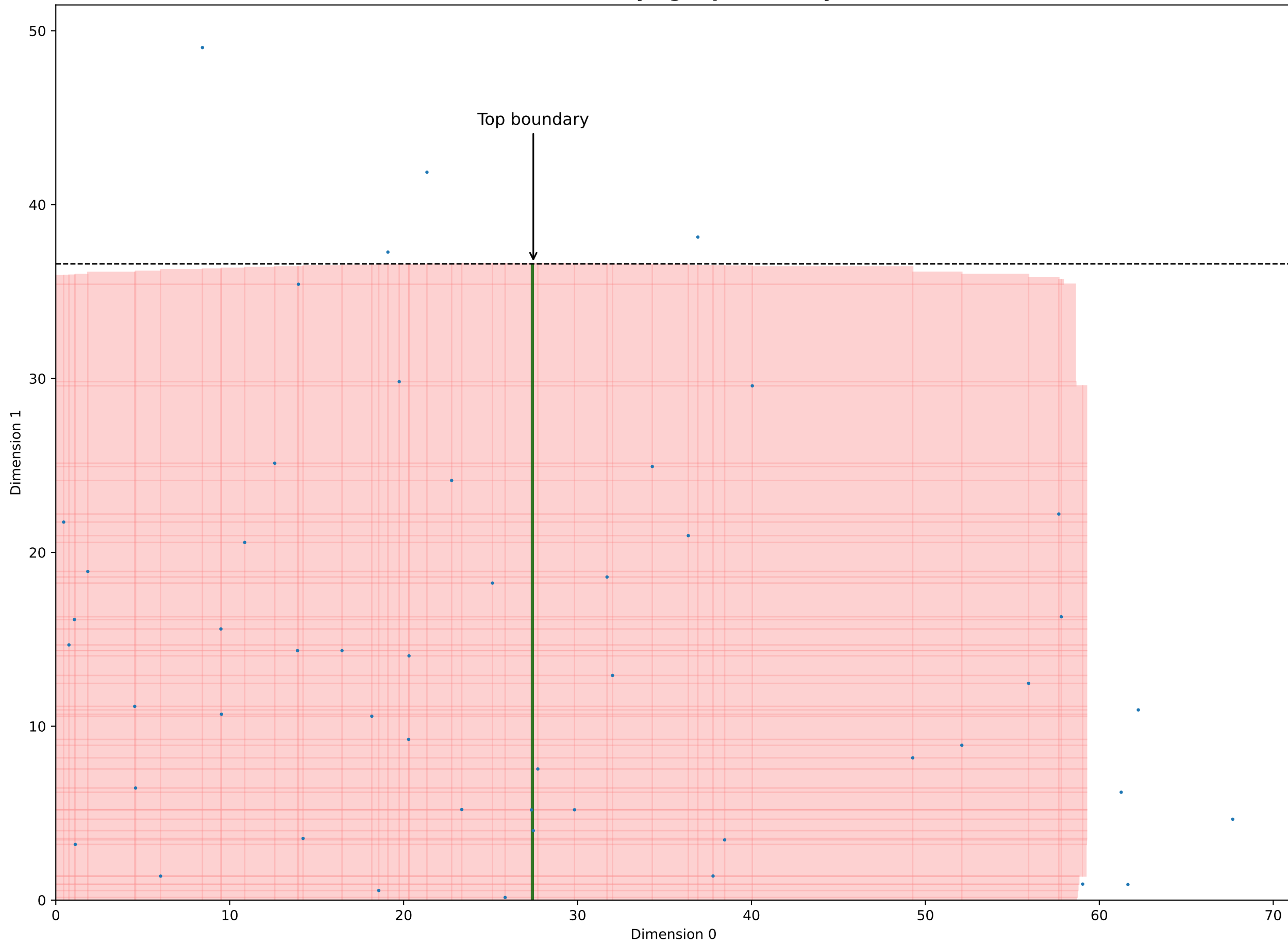
Vertical search: identifying top boundary (short-cut)
