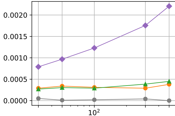
Runtime
