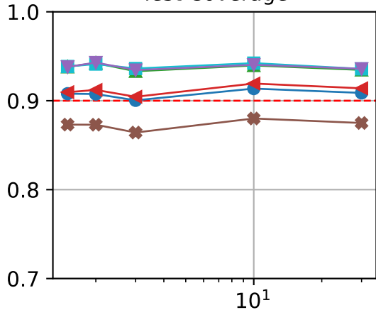
Test Coverage
