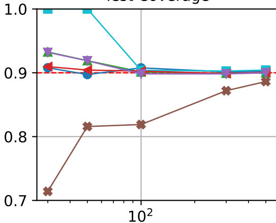
Test Coverage
