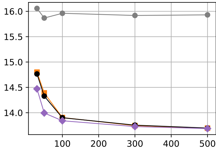
Dimension d = 10
