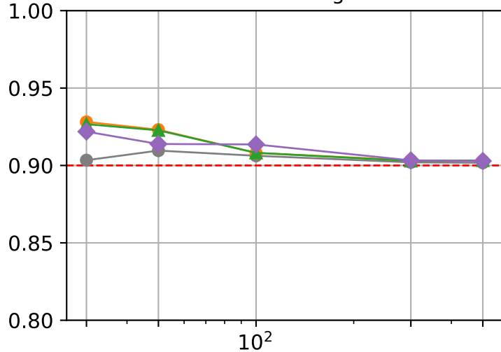
Test Coverage
