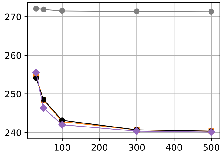
Dimension d = 100
