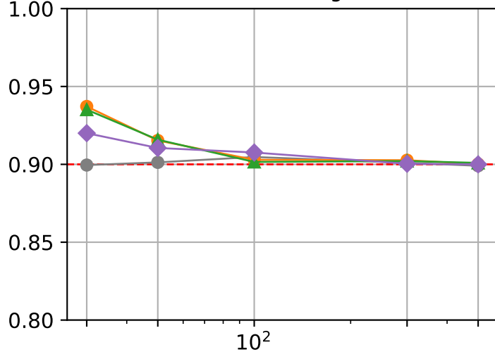
Test Coverage
