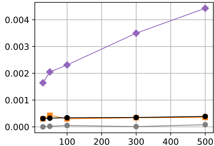
Dimension d = 4
