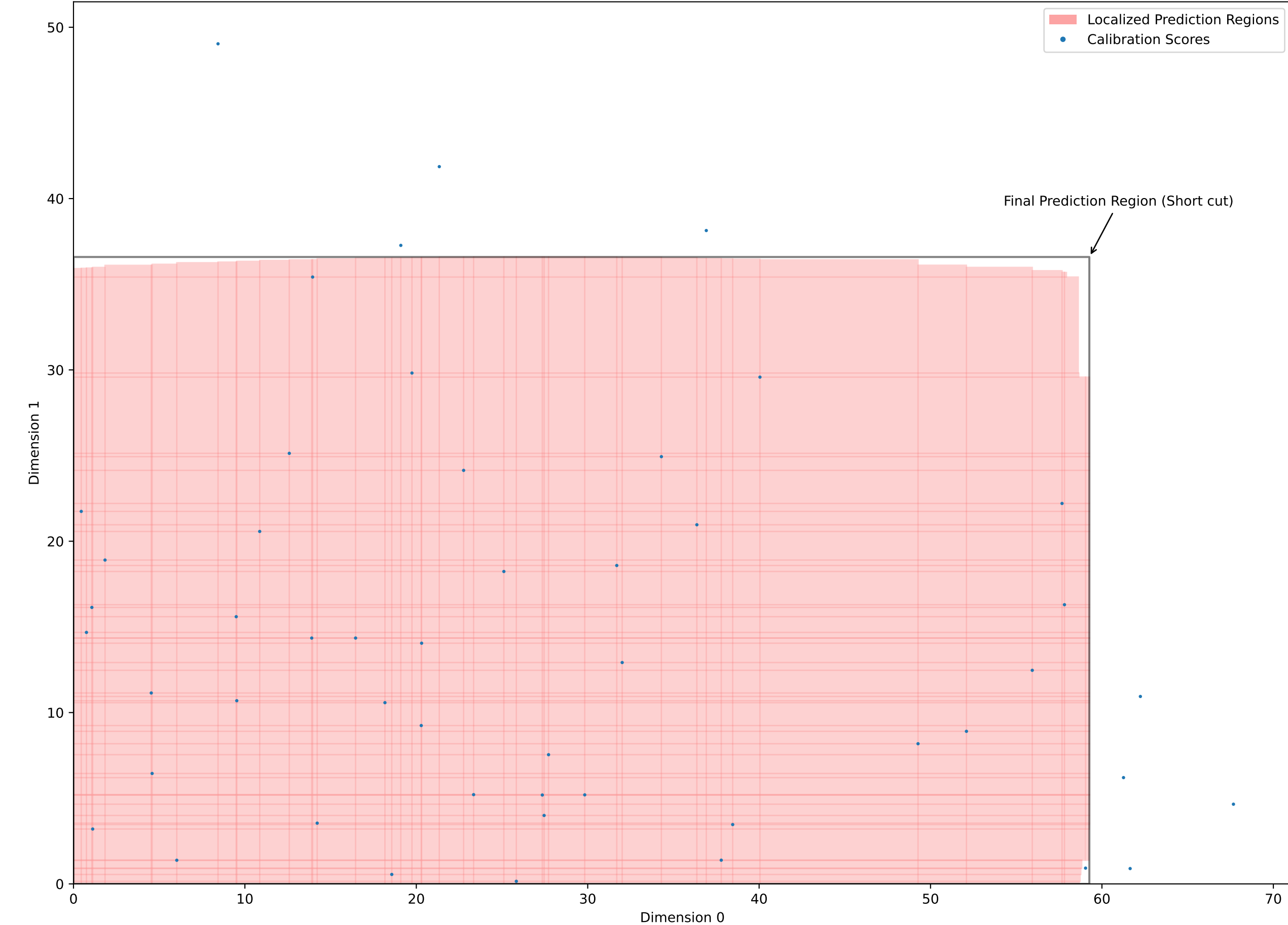
Full Prediction Region In The Score Space
