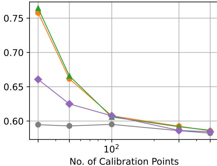
Volume (Log10)
