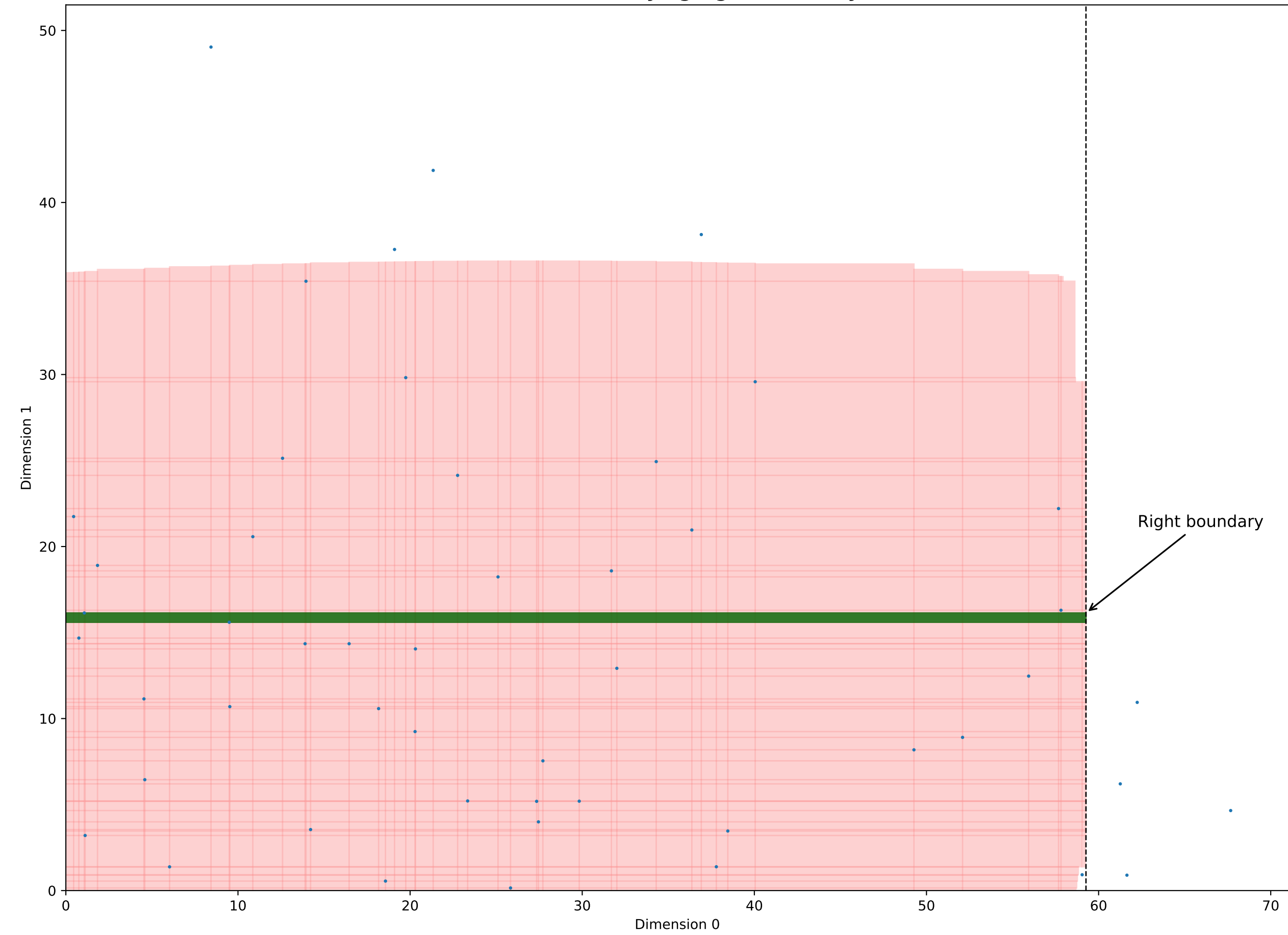
Horizontal search: identifying right boundary (short-cut)
