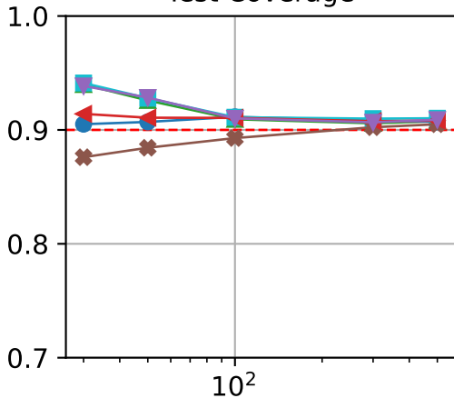
Test Coverage
