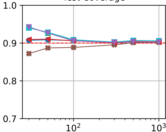
Test Coverage
