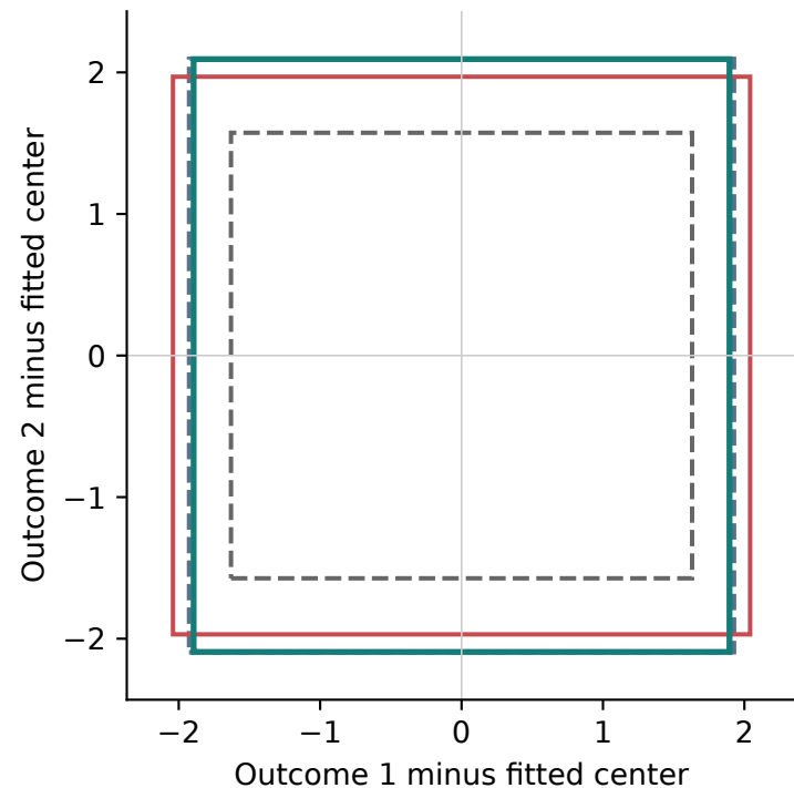
2d homoskedastic independent base alpha=0.1
