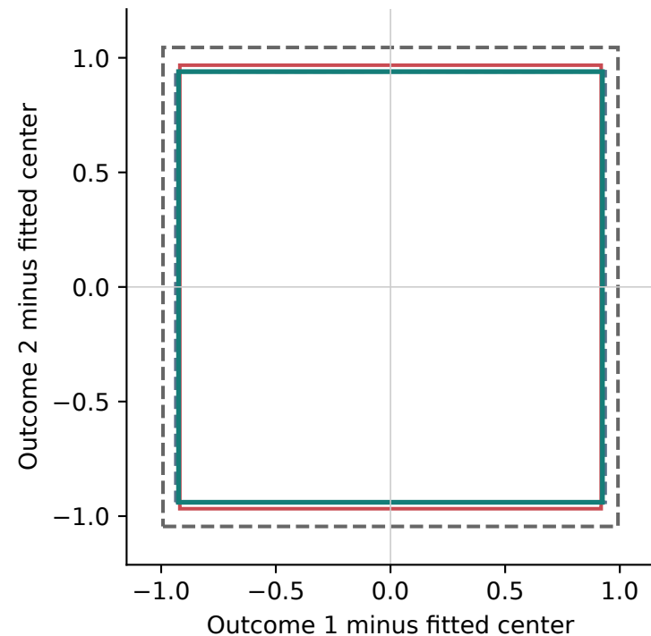
conservative signed 2d base alpha=0.02
