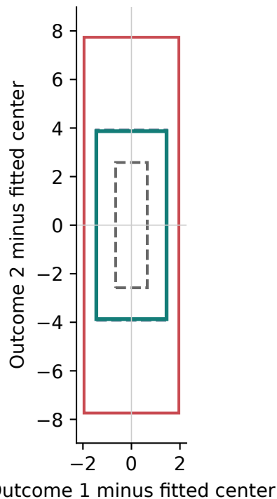
misspecified width base alpha=0.1
