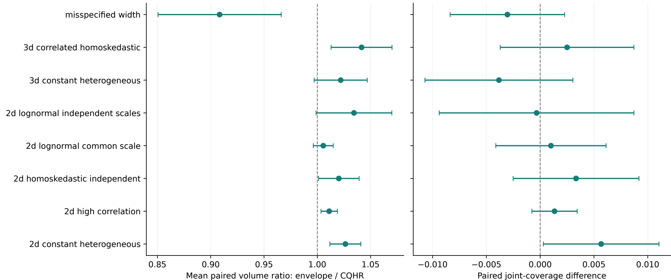
Fresh fitted toys: common base miscoverage 0.1; 95% Monte Carlo error bars
