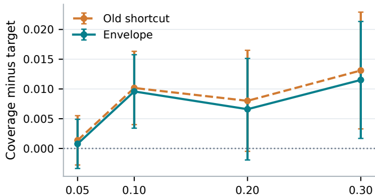
Gaussian
