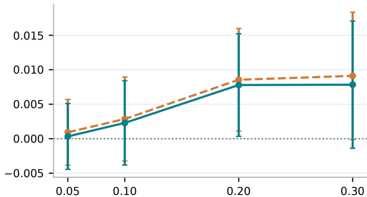
Laplace
