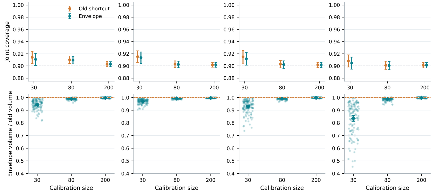
Gaussian
