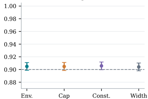
Laplace, 6 outcomes 90% marginal base
