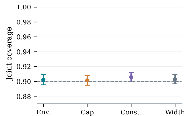
Gaussian, 2 outcomes 90% marginal base
