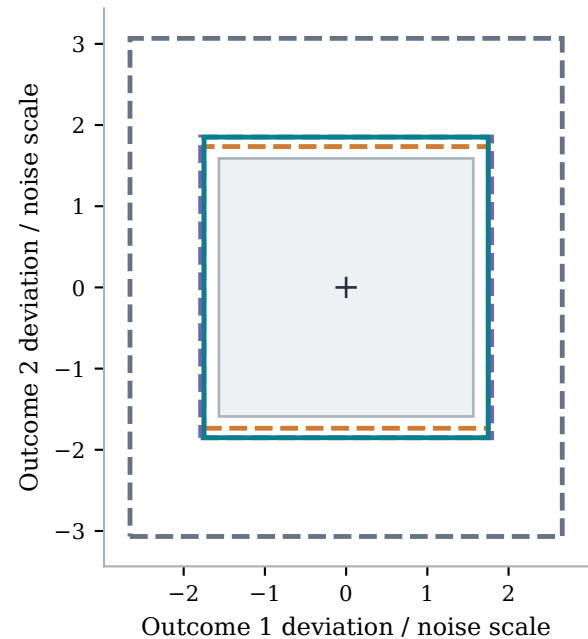
Gaussian, 2 outcomes: 90% marginal base
