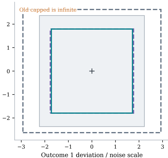
Gaussian, 2 outcomes: 98% marginal base
