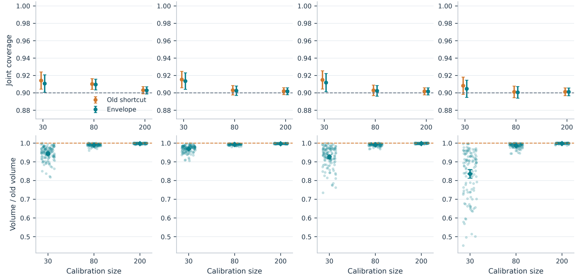
Gaussian
