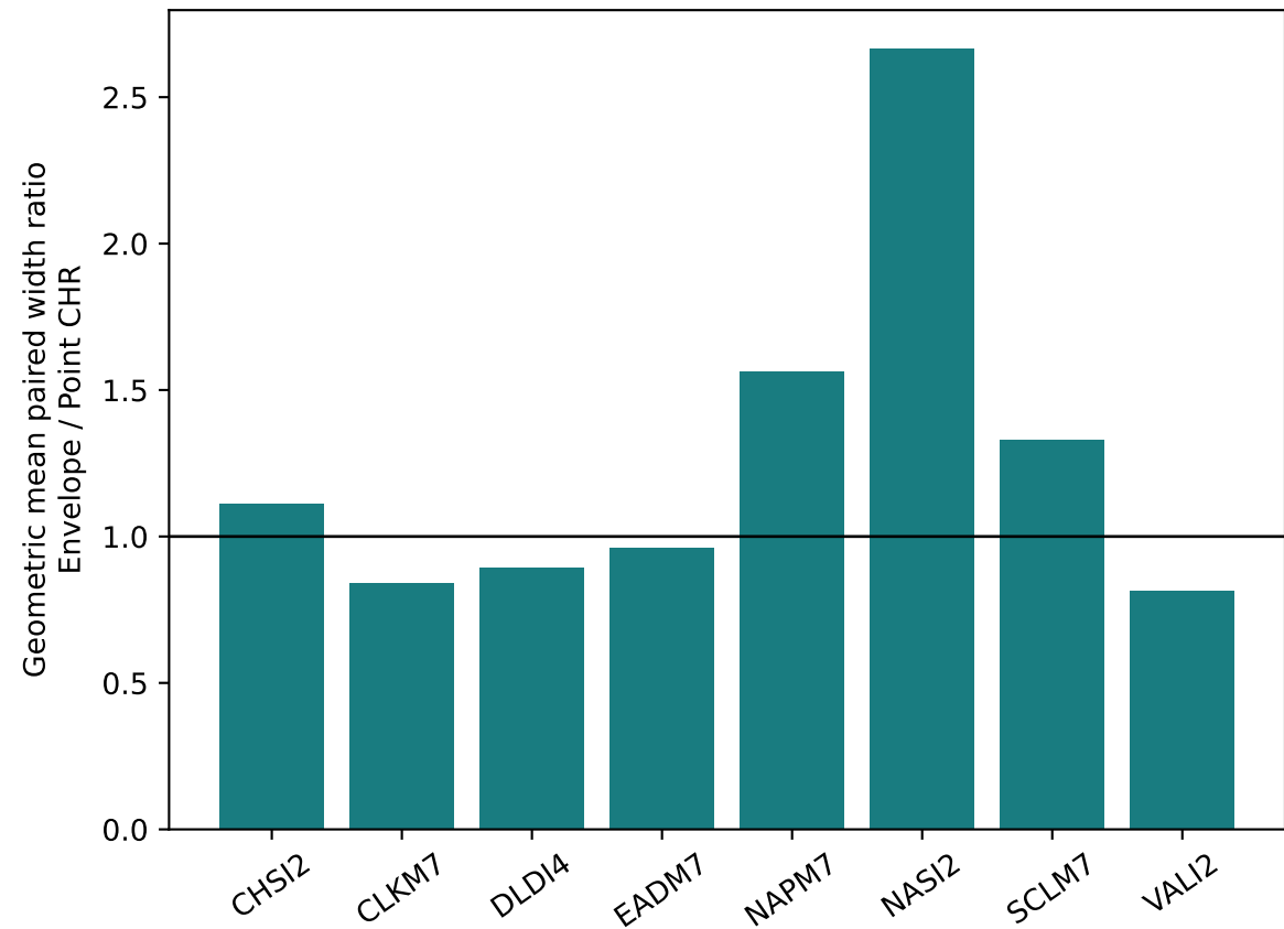
rf2: shape mismatch across eight coordinates | 200 paired splits
