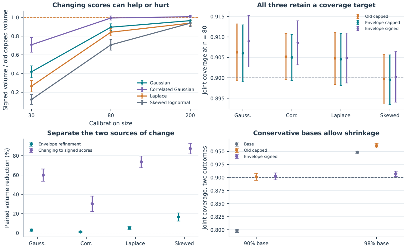
Figure 7: A score change is not the same as an envelope refinement. Top left: signed-envelope / old-capped paired volume ratios on finite pairs; crossing one means the signed version is larger. Top right: all-trial joint coverage at n = 80 . Bottom left: at n = 30 , the two comparisons are envelope-capped / old-capped and envelope-signed / envelope-capped, each using its own finite-pair denominator set. Their reductions are not additive. Bottom right: two-outcome Gaussian toys with 90% and 98% fitted marginal bases, both calibrated to a 90% joint target. All error bars are 95% Monte Carlo intervals across fitted trials.
