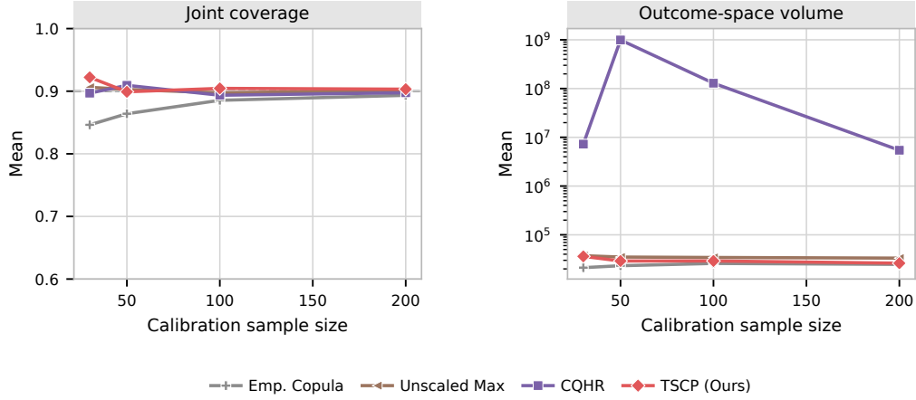
Figure 8: CQR experiment with d = 3 and base-interval miscoverage 0.5. TSCP uses capped nonnegative scores, Unscaled Max and Emp. Copula use raw signed scores, and CQHR uses its native quantile-hyperrectangle construction. Results are averaged over 30 independent repetitions.
