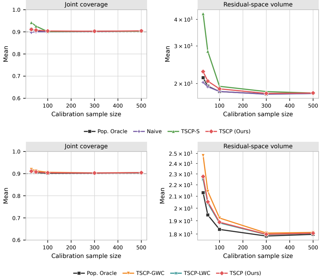
Figure S11: Performance of TSCP and alternative approaches on simulated data with d = 2 targets and heterogeneous Laplace noise. The target coverage level is 90%. Results are averaged over 200 trials. All methods achieve near-nominal coverage and approximate Pop. Oracle as the calibration sample size increases. TSCP tracks TSCP-LWC closely, with an almost indistinguishable average volume, highlighting the tightness of its rectangular enclosure.
