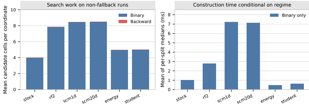
Figure 12: TSCP search work and construction time for 200 splits per real dataset at target coverage 0.9. Left: candidate cells inspected per coordinate, averaged over non-fallback runs. Counts include cells rejected by intersection checks. Right: whole-call construction times conditional on the observed regime, using the timing convention in Table 3. Unobserved regimes have no bars.
