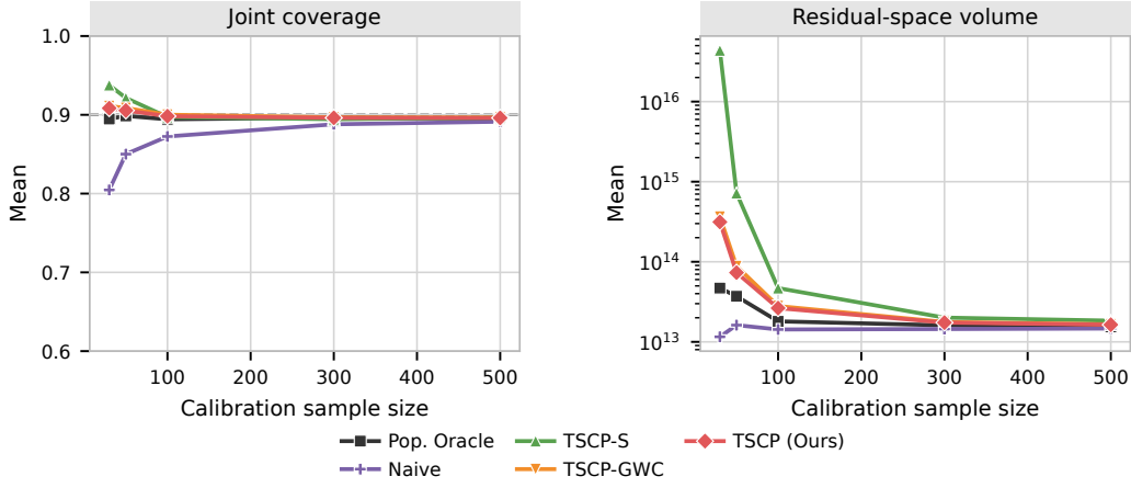
Figure S12: Performance of TSCP and alternative approaches on simulated data with d = 10 targets. Other details are as in Figure S11. TSCP-LWC is omitted from this figure due to its prohibitive cost with even moderately high-dimensional outcomes.
