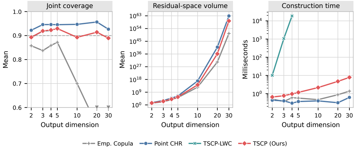
Figure S13: Absolute-residual experiment with Laplace noise, calibration size n = 30 , and varying output dimension d . Results are averaged over 30 repetitions. Panels report mean joint coverage, residual-space volume, and construction time in milliseconds. Volume and runtime use logarithmic axes. The dashed line marks target coverage 0.9; downward triangles identify coverage means below the displayed lower limit 0.6. TSCP-LWC is evaluated only at d \in \{2, 3, 4\} because of its rapidly increasing computational cost.
