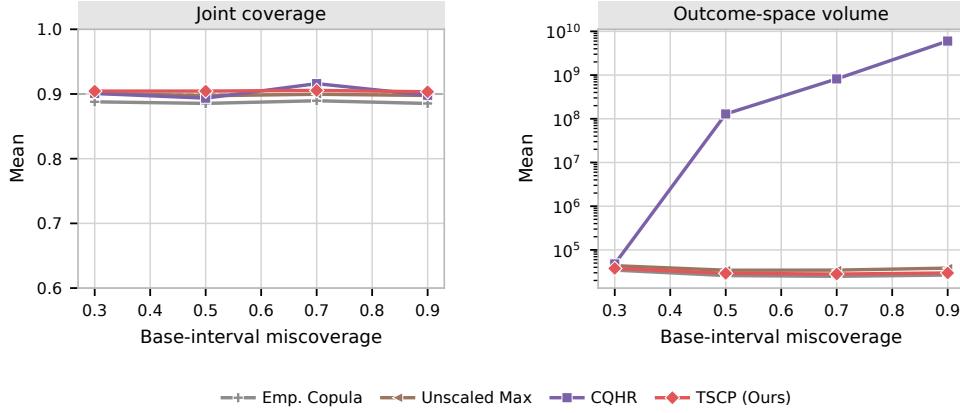
Figure S8: CQR sensitivity to the base-interval miscoverage with d = 3 , n = 100 , and final target coverage 0.9. TSCP uses capped scores, CQHR uses its native construction, and results average 30 independent repetitions.
