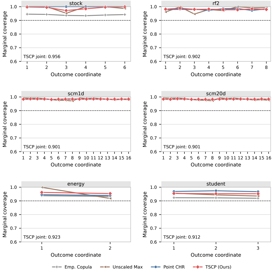
Figure S14: Coordinate-wise marginal coverage over 200 splits of each real dataset. The dashed line is the 0.9 joint target, and each panel also reports TSCP's mean joint coverage. Across-split standard deviations and pointwise Monte Carlo intervals are provided in the supplementary data. Coordinates follow the target-column order of each dataset.
