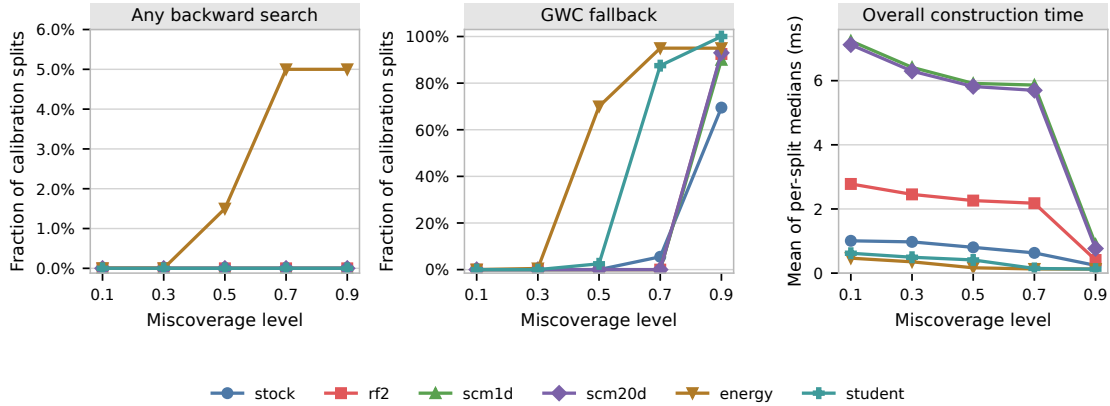
Figure S15: Computational stress sweep on the cached real-data calibration residuals. Each point summarizes 200 splits. The first two panels show the fractions of splits using any backward search or the global fallback; their vertical ranges differ. The final panel reports construction time. Additional miscoverage levels use the median of three uninstrumented calls per split; the main \alpha = 0.1 results use seven. All timing summaries average these per-split medians.
