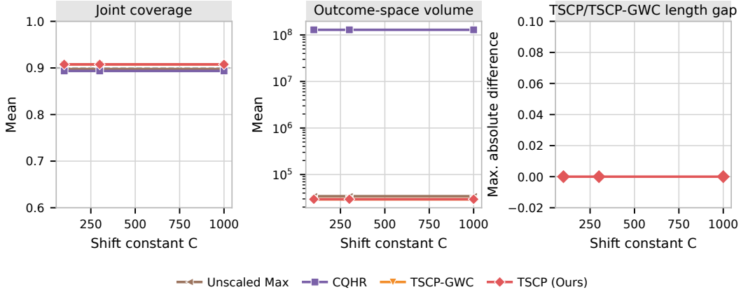
Figure S9: Sensitivity of shifted CQR scores to the additive constant C . The first two panels report coverage and mean outcome-space volume; the third reports the maximum coordinate-length difference between shifted TSCP and TSCP-GWC. Results use d = 3 , n = 100 , and 30 independent repetitions.
