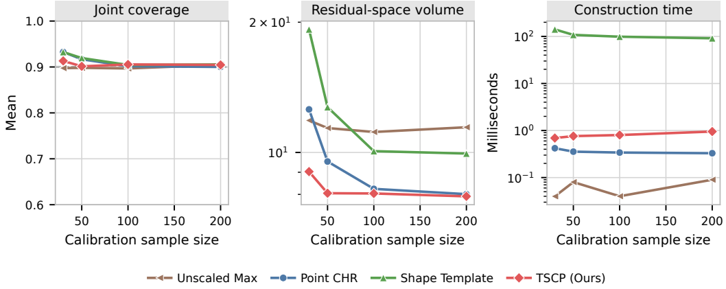
Figure S10: Comparison with a KDE/mean-shift hyperrectangular shape template for d = 2 Gaussian residuals with scales (2, 1) . Volume follows the same 2^{-d} normalization as the other residual-space experiments. Results average 100 independent repetitions, and runtime excludes the common regression fit.
