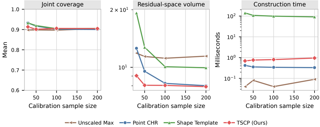
Figure S12: Comparison with a KDE/mean-shift hyperrectangular shape template for d = 2 Gaussian residuals with scales (2,1). Volume follows the same 2^{-d} normalization as the other residual-space experiments. Results average 100 independent repetitions, and runtime excludes the common regression fit.
