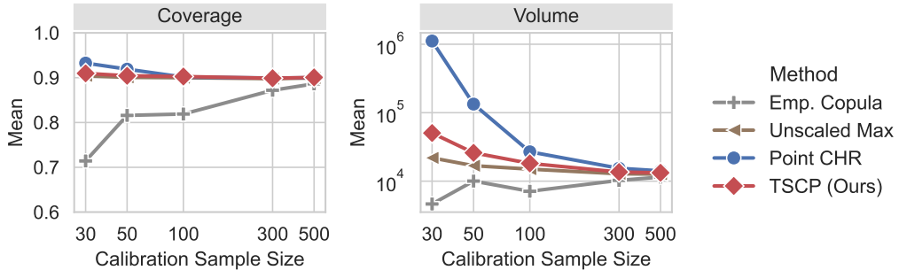
Figure S2: Average performance of the proposed TSCP method and alternative conformal prediction approaches in numerical experiments similar to those of Figure S1. Here, the outcome variables have homogeneous variance across their d = 10 dimensions, which gives an advantage to the Unscaled Max approach. The target coverage level is 0.9. TSCP attains near-nominal coverage and is competitive, while Unscaled Max is the most efficient in this homogeneous setting. Numerical results and corresponding standard deviations are reported in Table S5.
