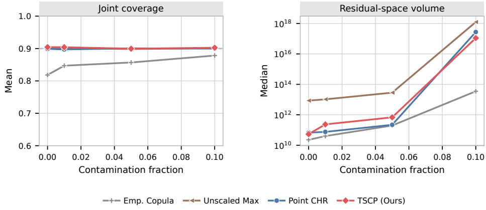
Figure S9: Row-wise contamination stress test with d = 10 and n = 100 . A contaminated observation has every noise coordinate multiplied by 10. The right panel reports median residual-space volume over 200 repetitions on a logarithmic scale.
