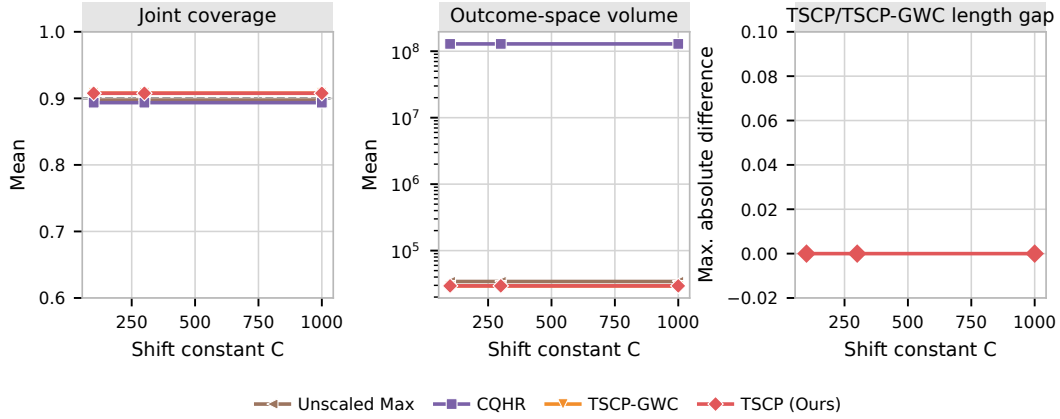
Figure S11: Sensitivity of shifted CQR scores to the additive constant C . The first two panels report coverage and mean outcome-space volume; the third reports the maximum coordinate-length difference between shifted TSCP and TSCP-GWC. Results use d = 3 , n = 100 , and 30 independent repetitions.
