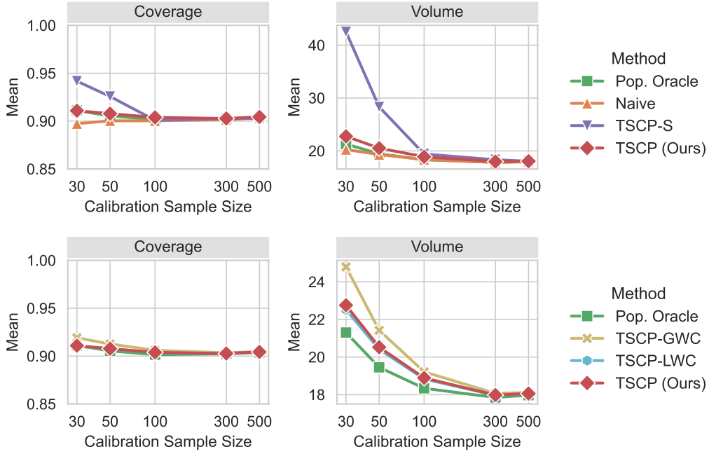
Figure S13: Performance of TSCP and alternative approaches on simulated data with d = 2 targets and heterogeneous Laplace noise. The target coverage level is 90%. Results are averaged over 200 trials. All methods achieve near-nominal coverage and approximate Pop. Oracle as the calibration sample size increases. TSCP tracks TSCP-LWC closely, with an almost indistinguishable average volume, highlighting the tightness of its rectangular enclosure.
