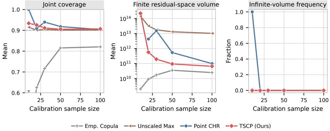
Figure S6: Small-calibration-sample stress test with independent Gaussian noise and scales (10, 9, \dots, 1) . The middle panel averages only finite residual-space volumes; the right panel reports the fraction of repetitions with infinite volume. A downward triangle at the lower plotting boundary marks the Emp. Copula mean below 0.6. Results average 200 repetitions.
