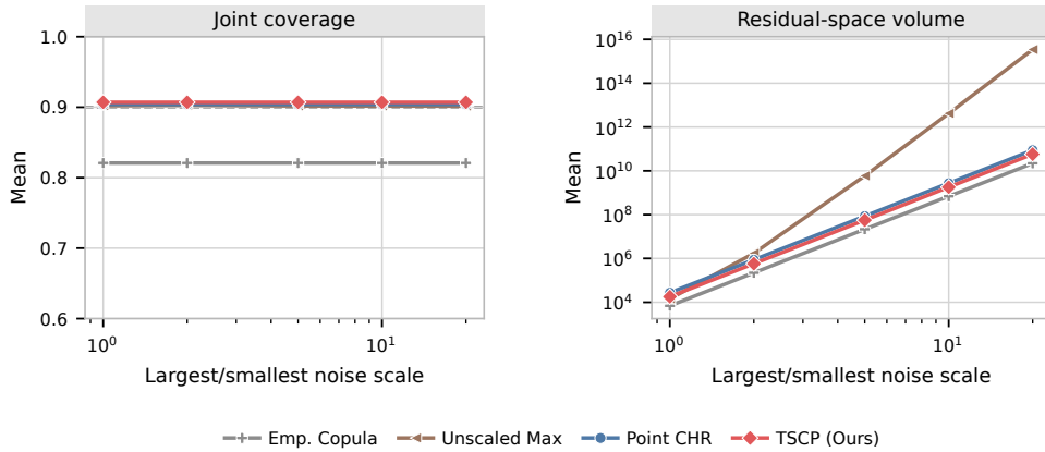
Figure S4: Sensitivity to the ratio between the largest and smallest outcome noise scales, with independent Gaussian errors and n = 100 . The scales are geometrically spaced, and both axes of the volume panel are logarithmic. Results average 200 repetitions.
