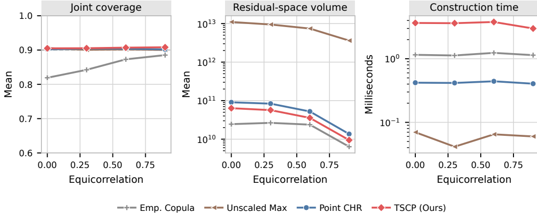
Figure S3: Sensitivity to equicorrelated Gaussian noise at d = 10 and n = 100 . The three panels report joint coverage, mean residual-space volume, and mean construction time. Results average 200 repetitions; the dashed line marks the target coverage.
