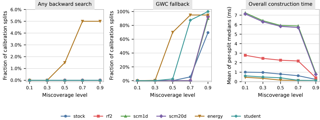
Figure S17: Computational stress sweep on the cached real-data calibration residuals. Each point summarizes 200 splits. The first two panels show the fractions of splits using any backward search or the global fallback; their vertical ranges differ. The final panel reports construction time. Additional miscoverage levels use the median of three uninstrumented calls per split; the main \alpha = 0.1 results use seven. All timing summaries average these per-split medians.
