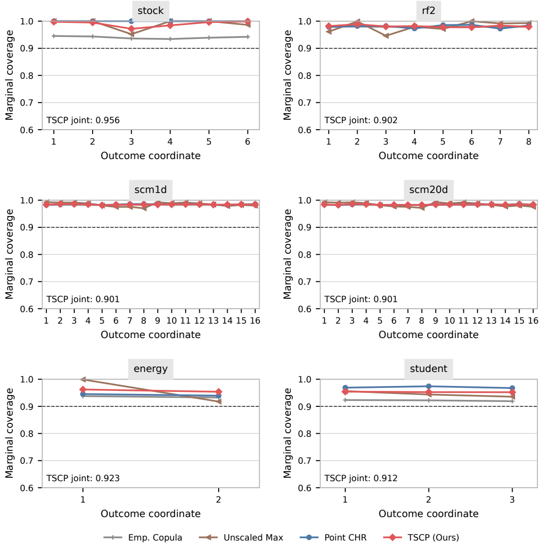
Figure S16: Coordinate-wise marginal coverage over 200 splits of each real dataset. The dashed line is the 0.9 joint target, and each panel also reports TSCP's mean joint coverage. Across-split standard deviations and pointwise Monte Carlo intervals are provided in the supplementary data. Coordinates follow the target-column order of each dataset.
