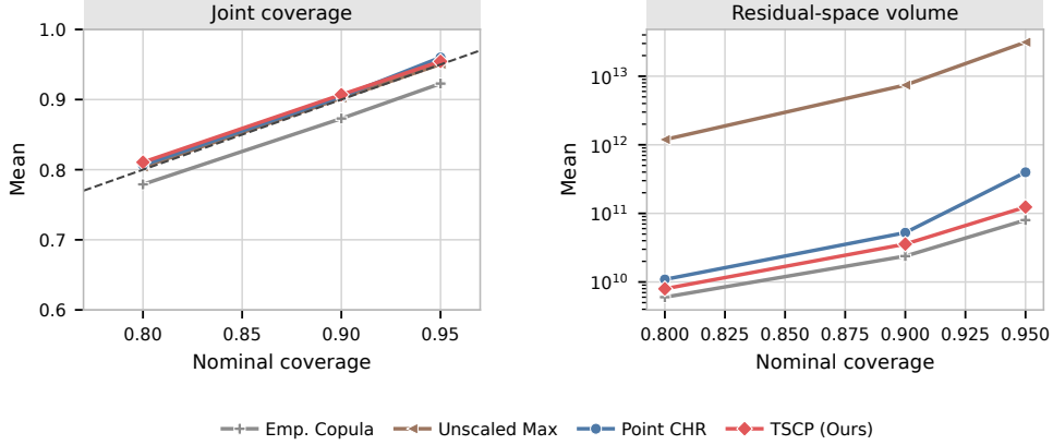
Figure S5: Sensitivity to the nominal coverage level in the d = 10 equicorrelated Gaussian experiment with n = 100 and \rho = 0.6 . The dashed diagonal in the left panel is exact nominal calibration. Results average 200 repetitions.
