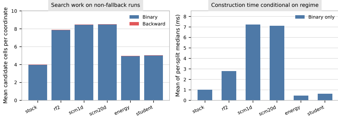
Figure 10: TSCP search work and construction time for 200 splits per real dataset at target coverage 0.9. Left: candidate cells inspected per coordinate, averaged over non-fallback runs. Counts include cells rejected by intersection checks. Right: whole-call construction times conditional on the observed regime, using the timing convention in Table 3. Unobserved regimes have no bars.
