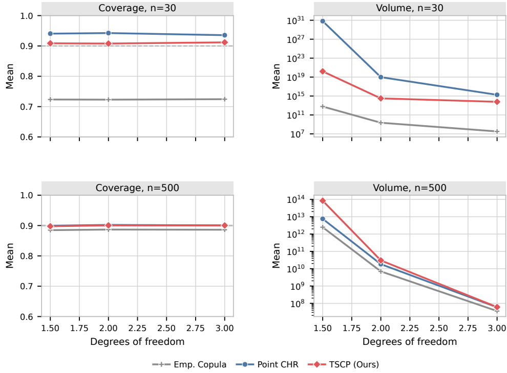
Figure S7: Coverage and mean residual-space volume under independent, common-scale Student t noise for d = 10 . The top row uses n = 30 calibration examples and the bottom row uses n = 500 . Results average 200 repetitions; volume is shown on a logarithmic scale.
