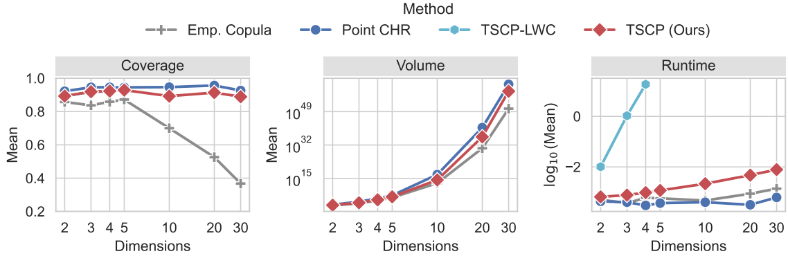
Figure S15: Performance of TSCP and alternative approaches on simulated data with fixed sample size |\mathcal{D}_{\text{cal}}| = 30 , as a function of the number of output dimensions d . Other details are as in Figure S13. These results are averaged over 30 repetitions under the fixed-pool protocol. The runtime results are presented in seconds on a \log_{10} scale. The runtime of all methods except TSCP-LWC scales well with number of dimensions. TSCP-LWC is only applied when d \in \{2, 3, 4\} due to the exponential growth of its runtime.
