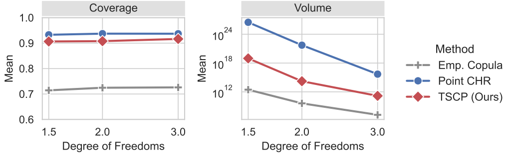
(a) Small sample, |\mathcal{D}_{\text{cal}}| = 30 . Output dimensions d = 10 .
