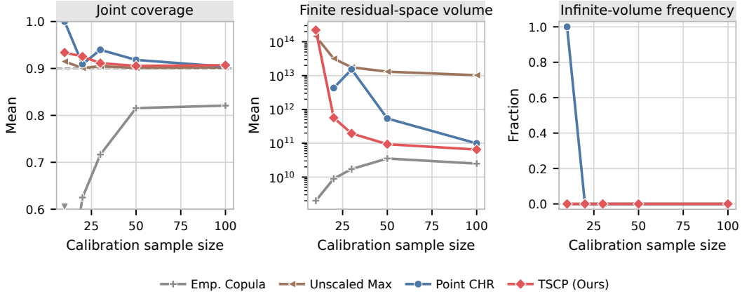
Figure S4: Small-calibration-sample stress test with independent Gaussian noise and scales (10, 9, \dots, 1) . The middle panel averages only finite residual-space volumes; the right panel reports the fraction of repetitions with infinite volume. A downward triangle at the lower plotting boundary marks the Emp. Copula mean below 0.6. Results average 200 repetitions.
