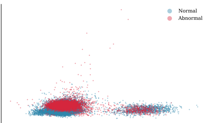
PC1+PC2 explain 19.9% of variance LOGMEL — PCA
