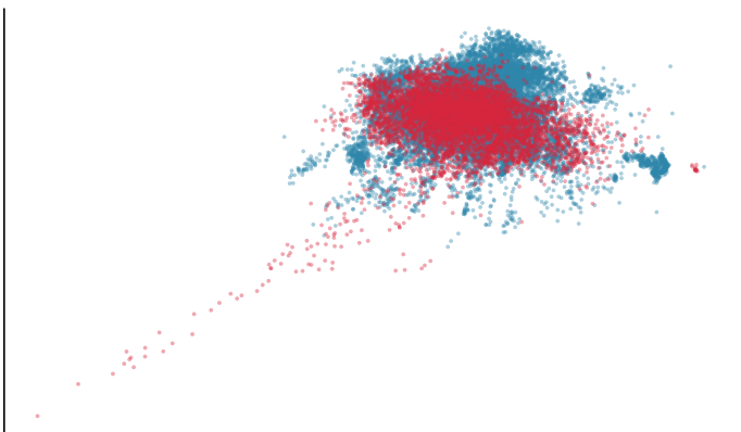
PC1+PC2 explain 44.8% of variance PWP — PCA
