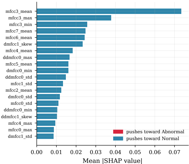
rf_mfcc — top 20 features by mean |SHAP|
