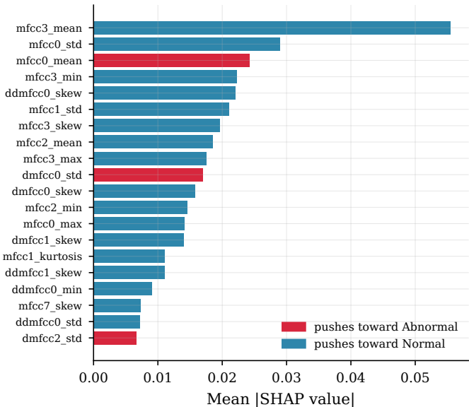
svm_mfcc — top 20 features by mean |SHAP|
