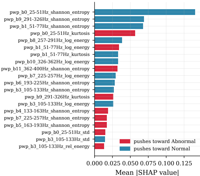
svm_pwp — top 20 features by mean |SHAP|
