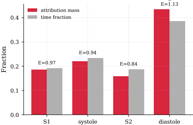
CNN Grad-CAM: attribution mass vs. time budget
