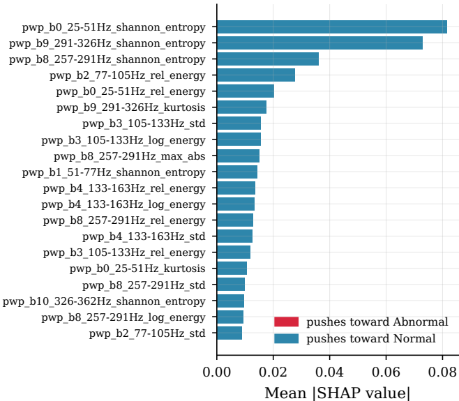
rf_pwp — top 20 features by mean |SHAP|
