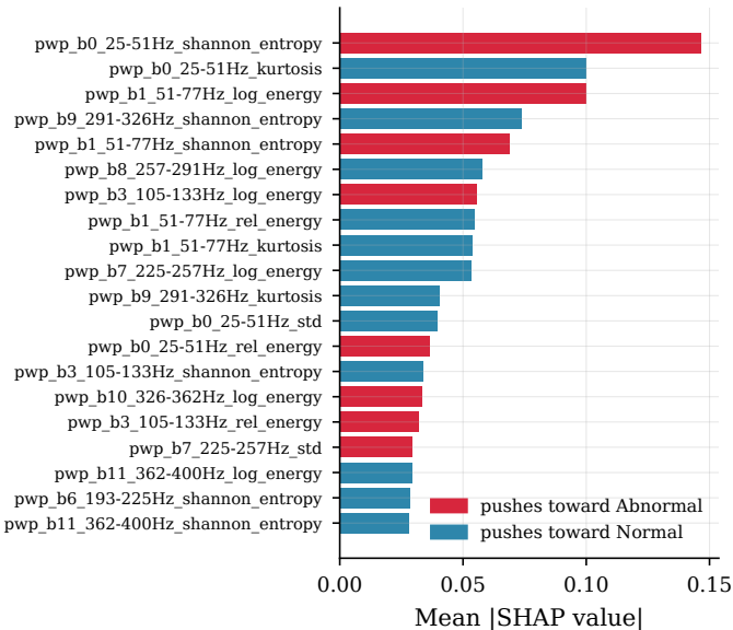
svm_pwp — top 20 features by mean |SHAP|
