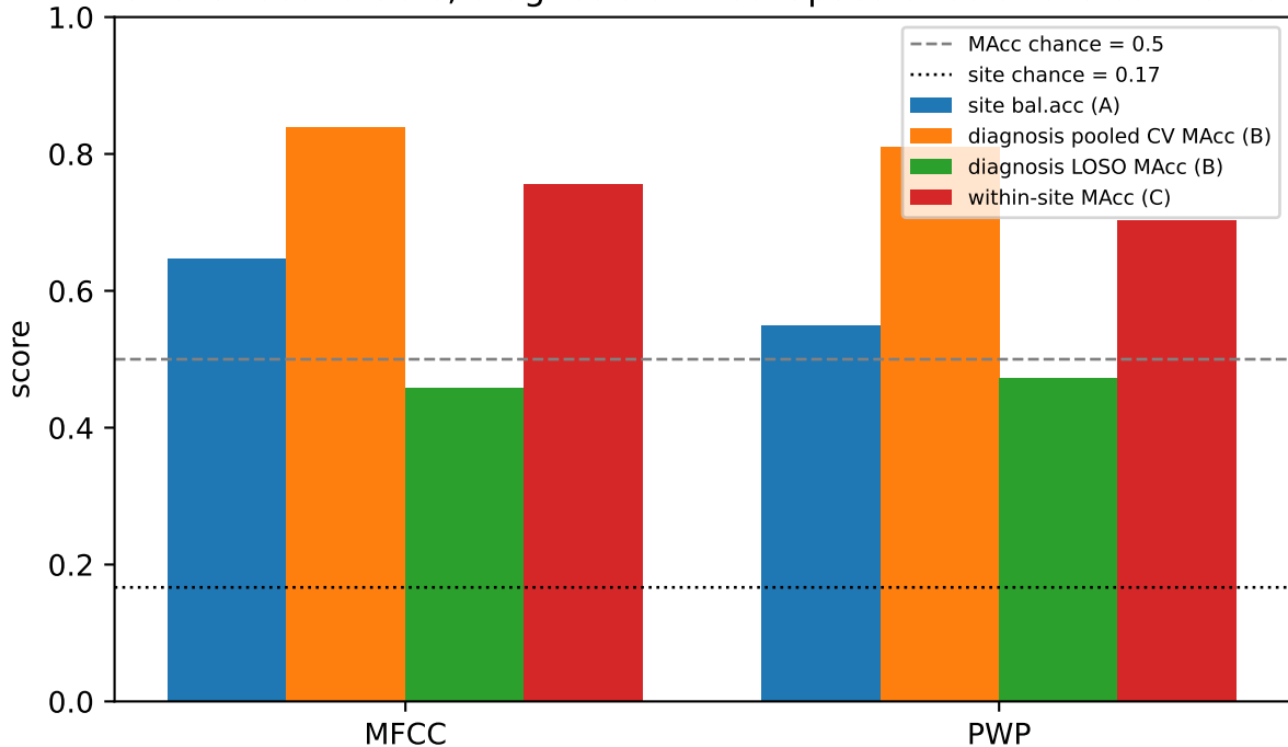
Site is recoverable; diagnosis skill collapses once site is controlled
