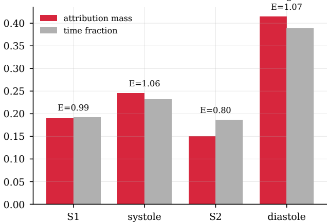
CNN Grad-CAM: attribution mass vs. time budget
