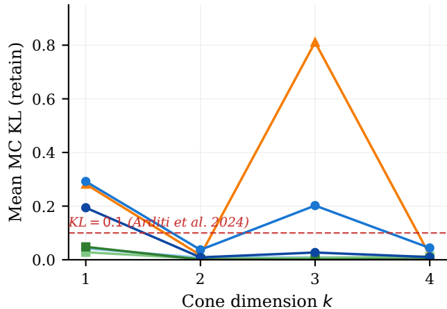
(b) KL falls below surgicality threshold at k=2
