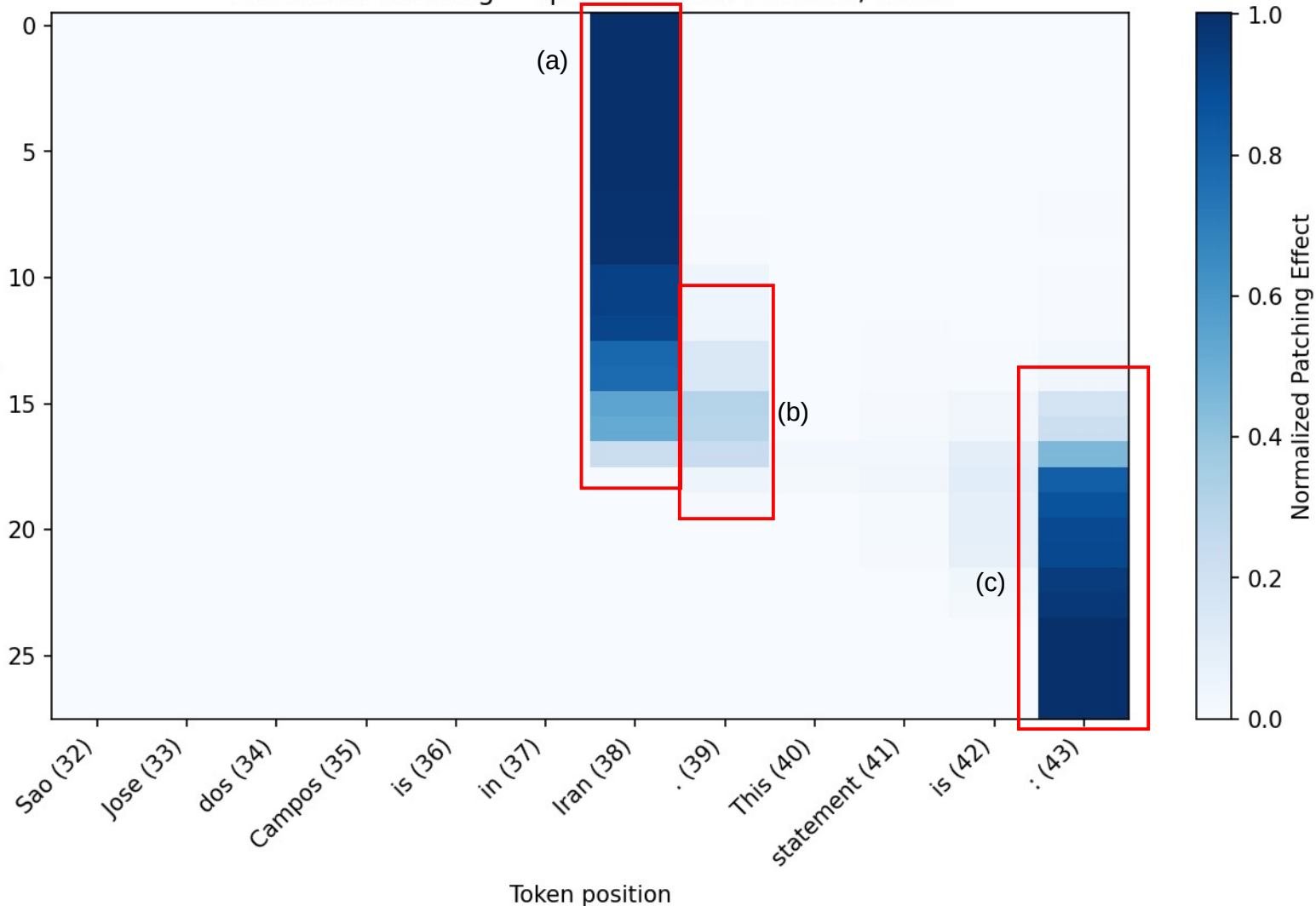
Activation Patching — qwen-2.5-1.5b-instruct / cities
