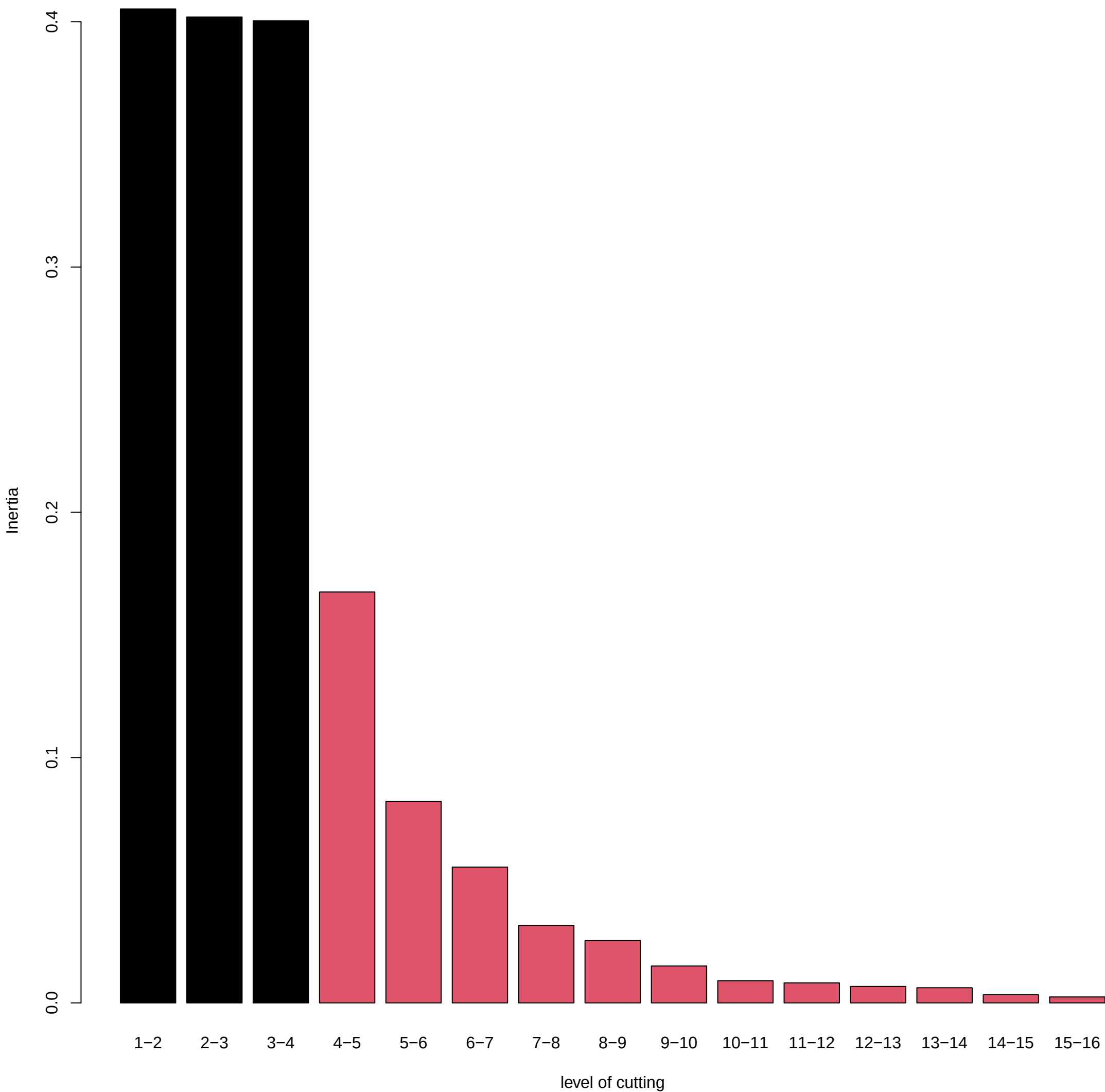
Inter-cluster inertia gains
