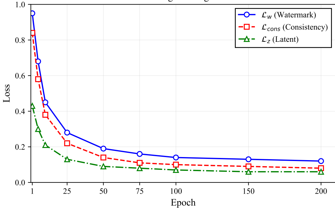
Training Convergence
