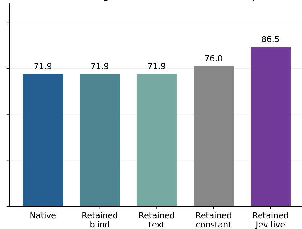
ARC-Challenge science: 25/96 routed to repair
