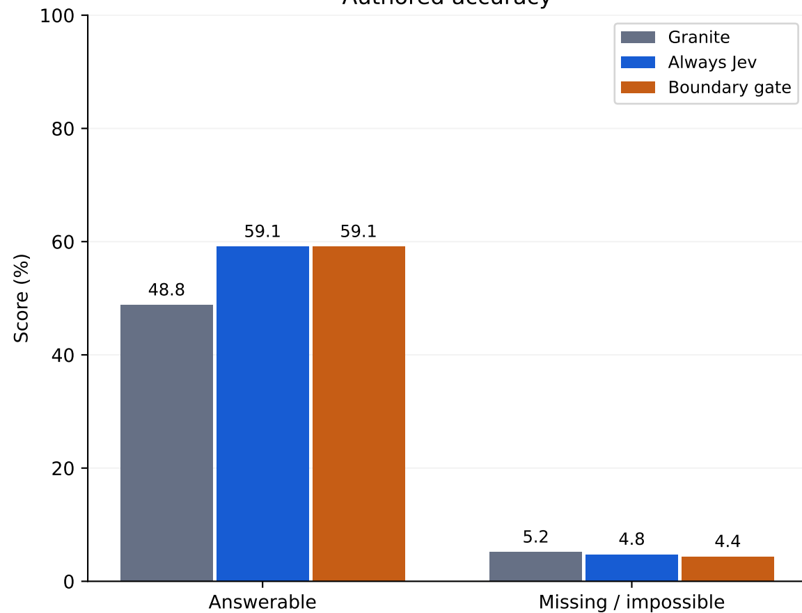
Authored accuracy
